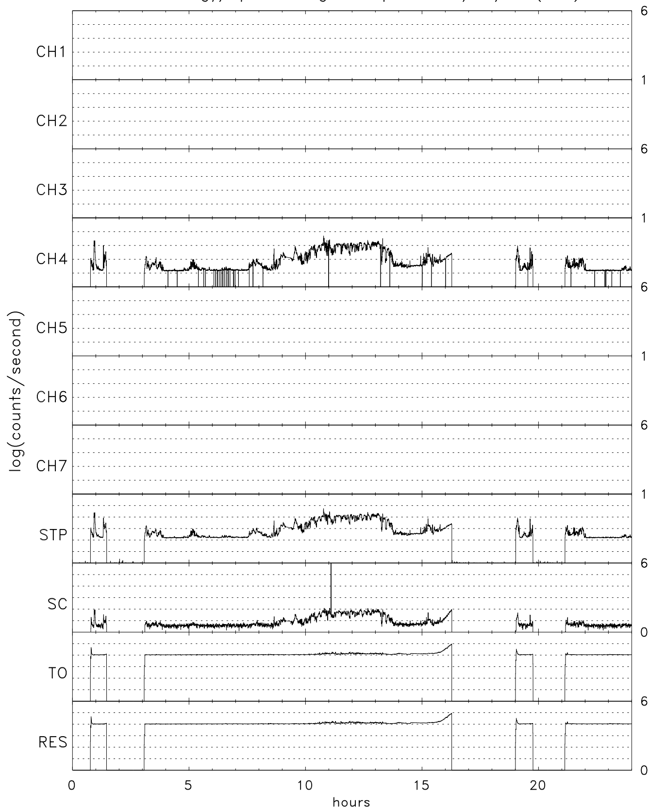
TIDE energy/spin averaged Stops for 01/17/07 (017)
