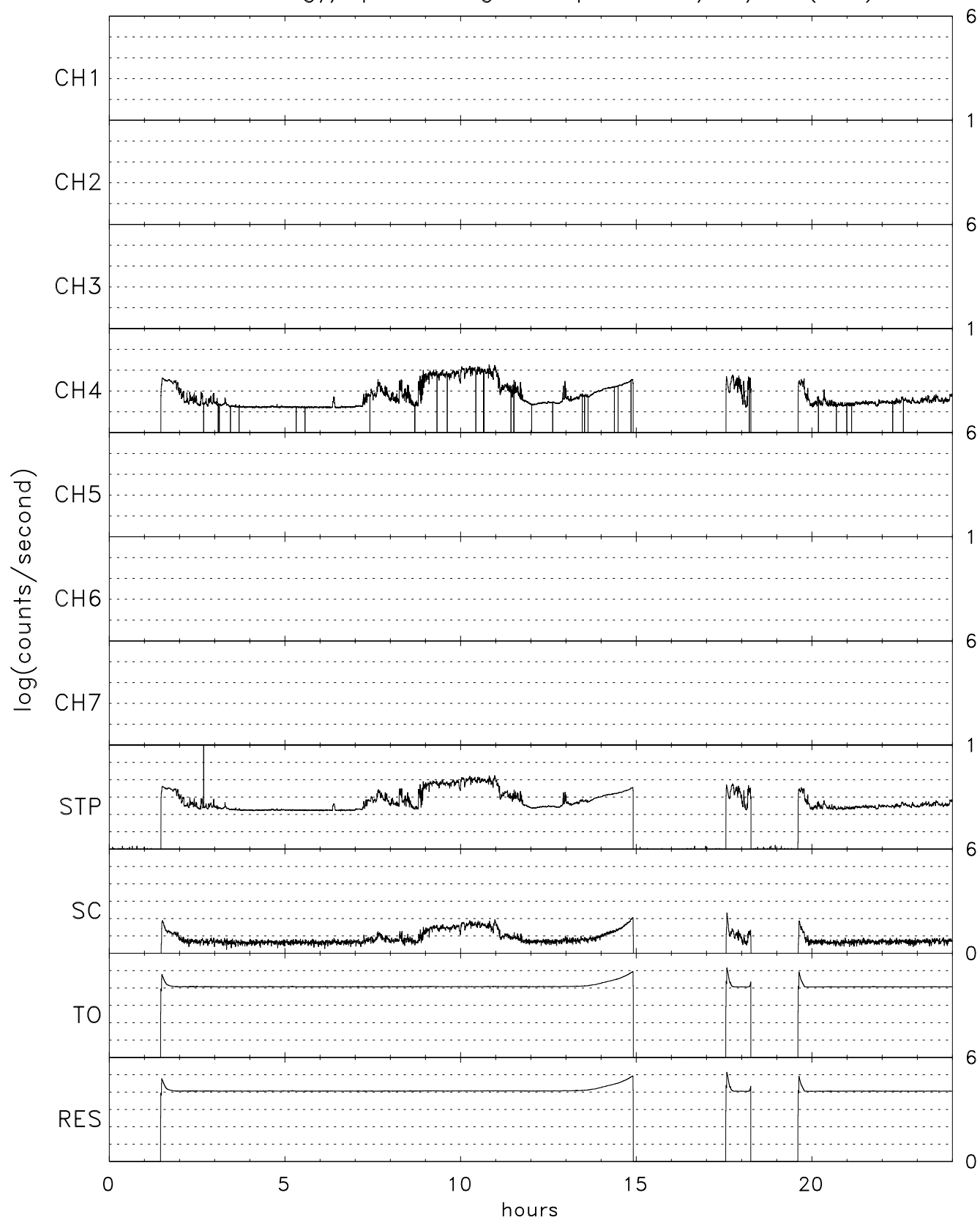
TIDE energy/spin averaged Stops for 01/14/07 (014)
