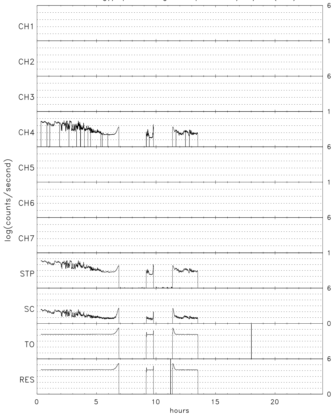
TIDE energy/spin averaged Stops for 01/09/07 (009)
