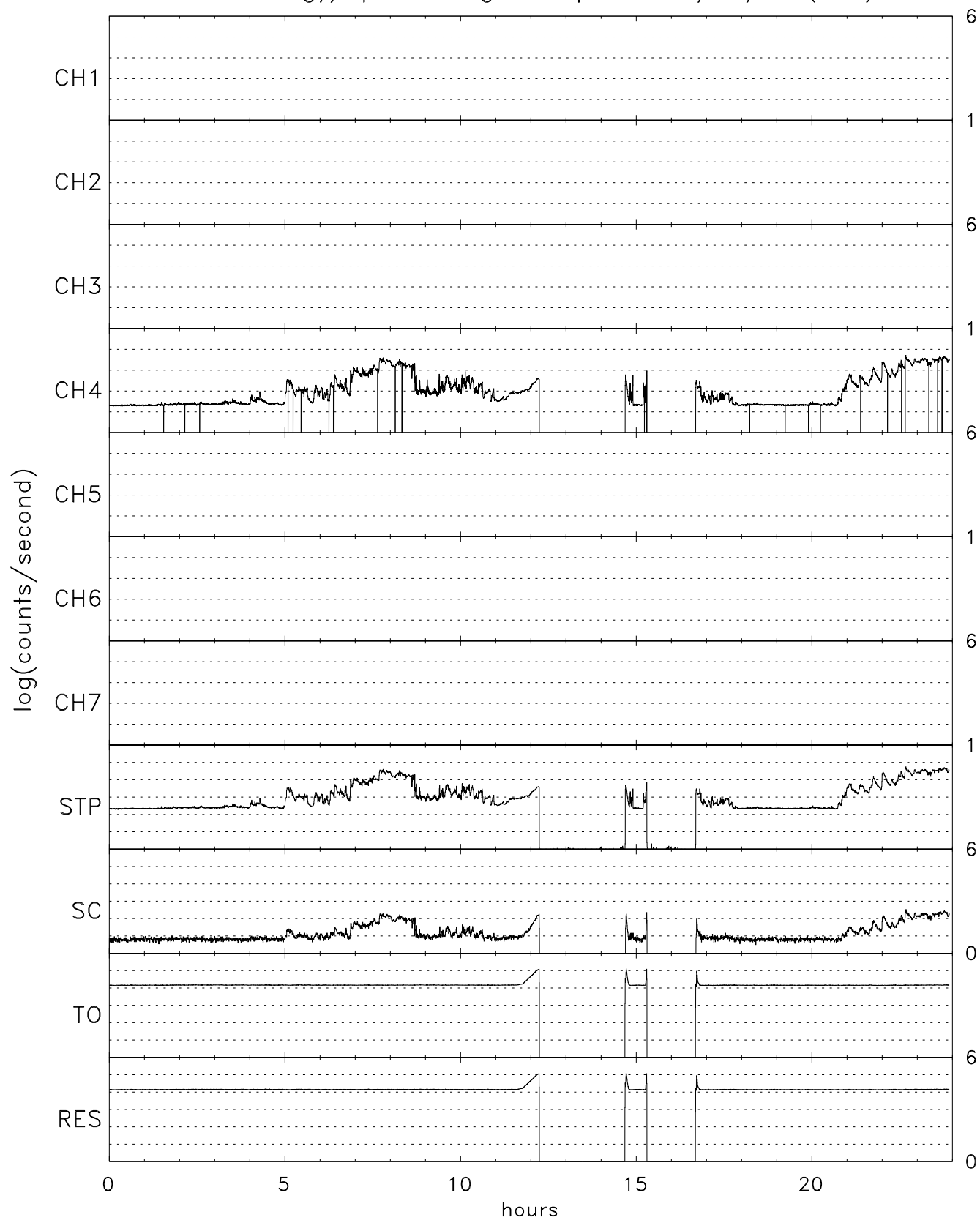
TIDE energy/spin averaged Stops for 01/08/07 (008)
