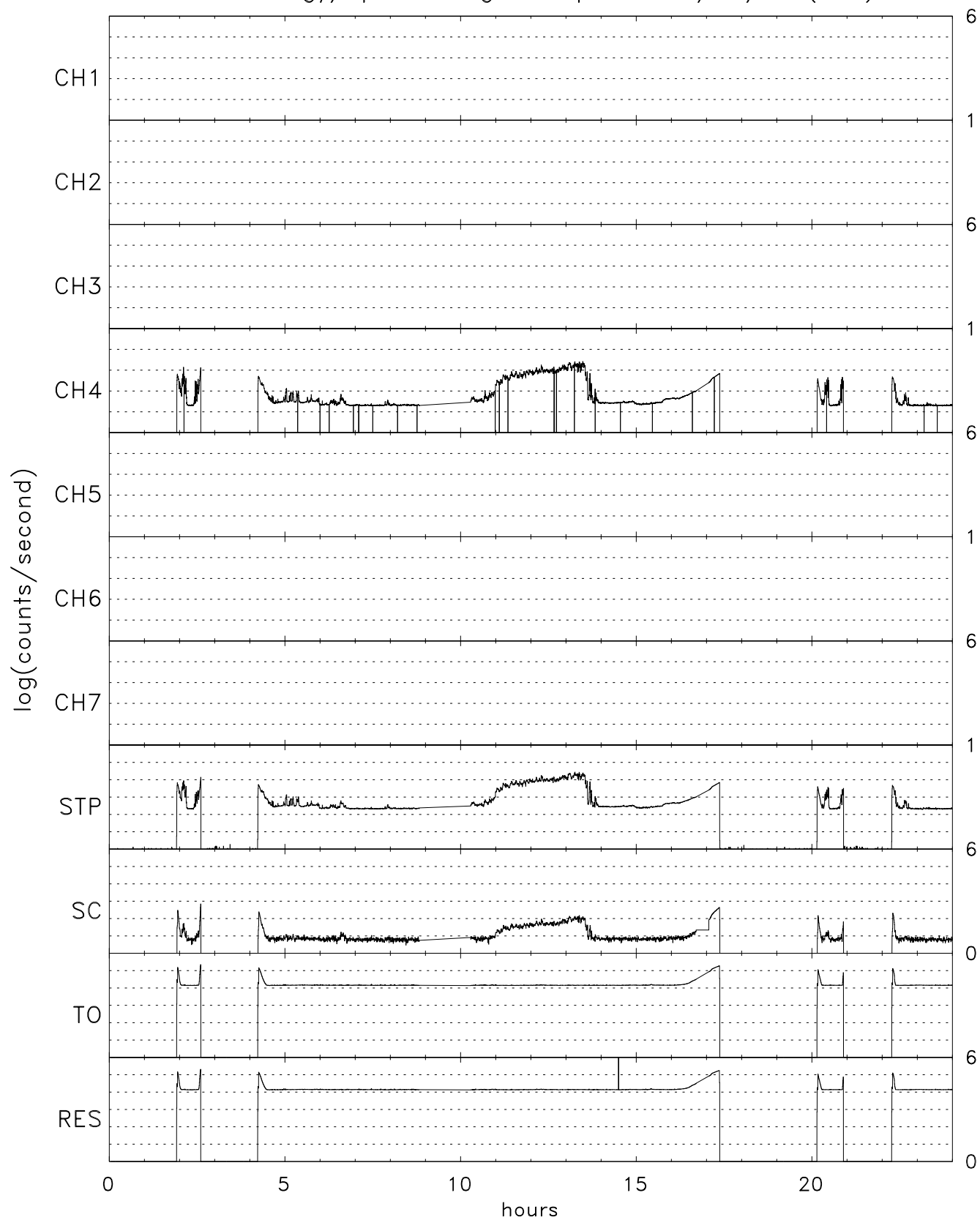
TIDE energy/spin averaged Stops for 01/07/07 (007)
