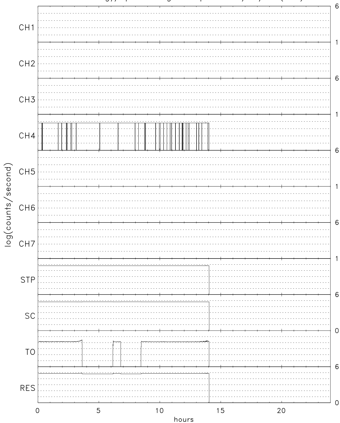
TIDE energy/spin averaged Stops for 01/03/07 (003)
