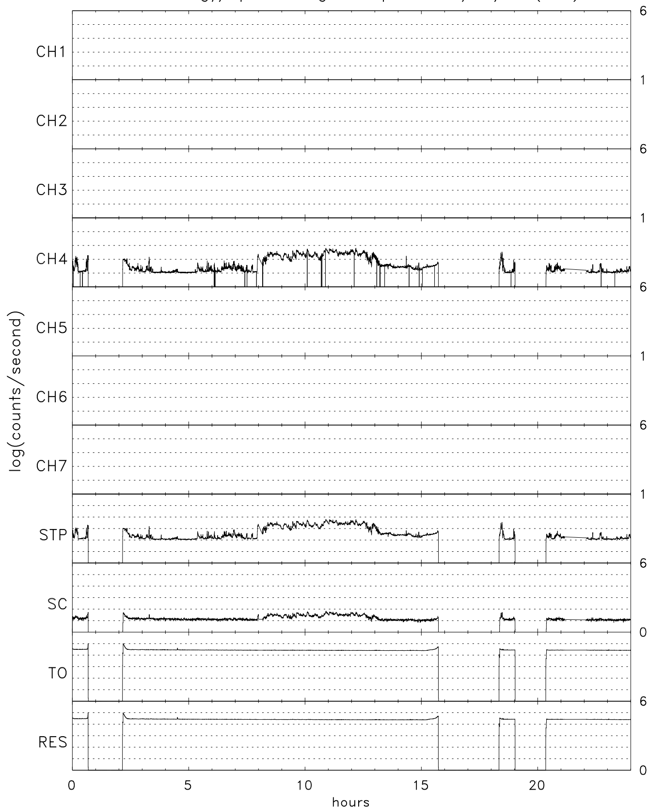
TIDE energy/spin averaged Stops for 12/22/06 (356)
