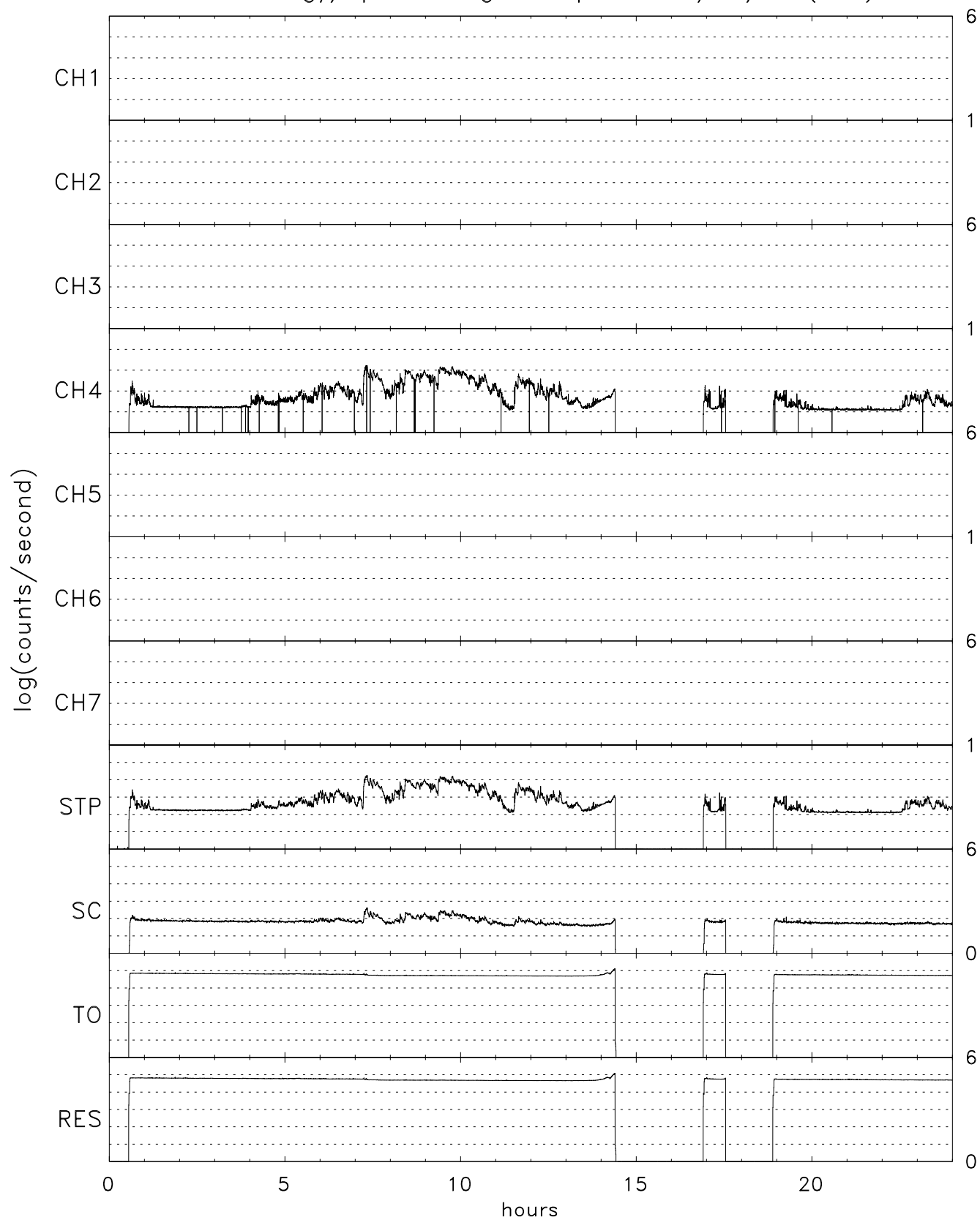
TIDE energy/spin averaged Stops for 12/19/06 (353)
