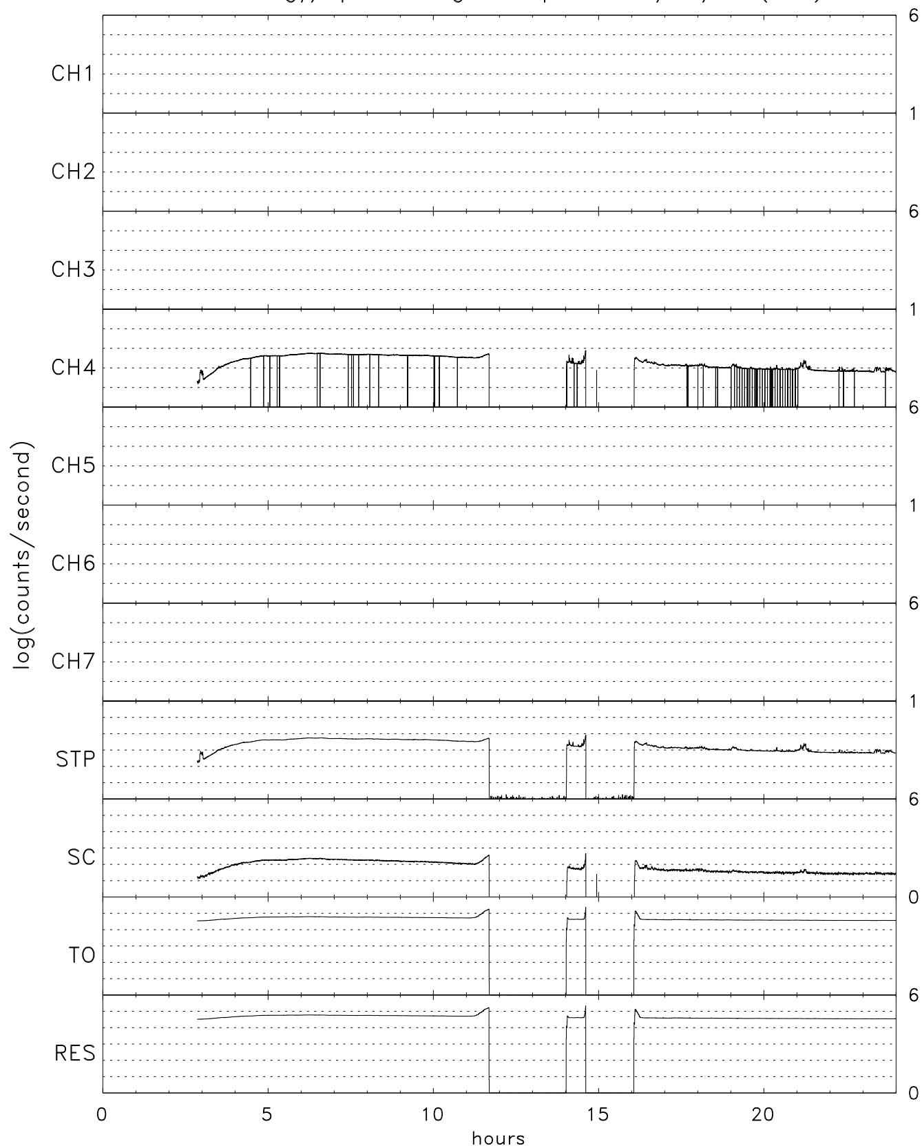
TIDE energy/spin averaged Stops for 12/13/06 (347)
