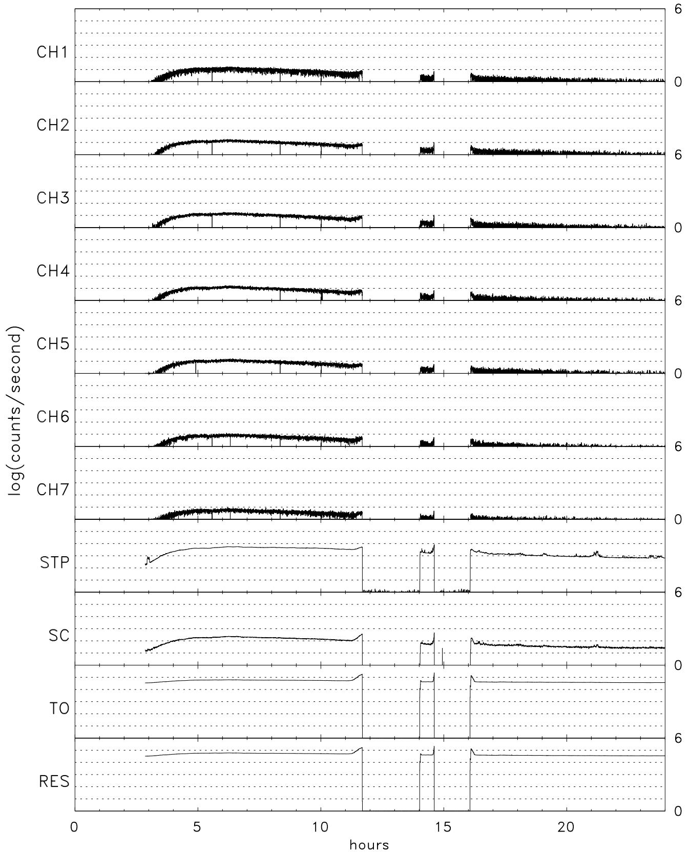
TIDE energy/spin averaged H+ for 12/13/06 (347)
