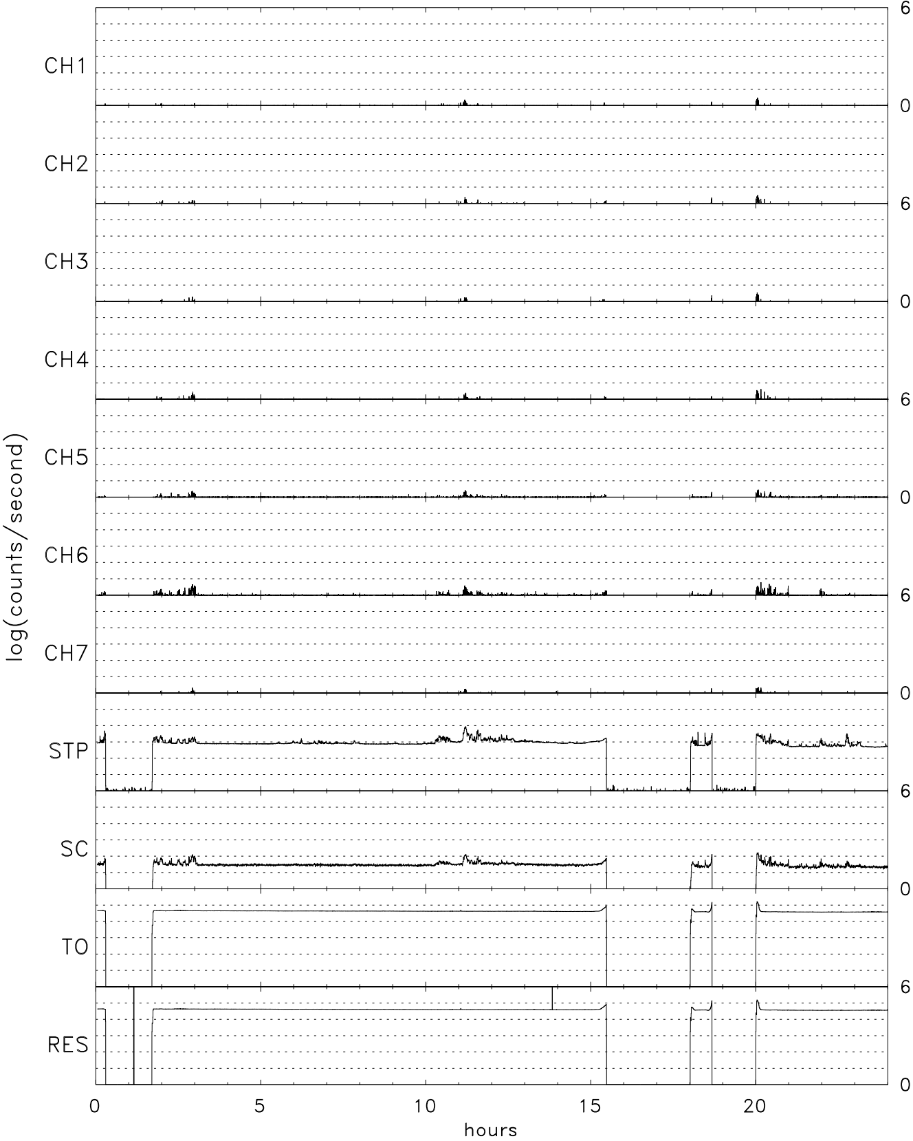
TIDE energy/spin averaged 0+ for 12/09/06 (343)
