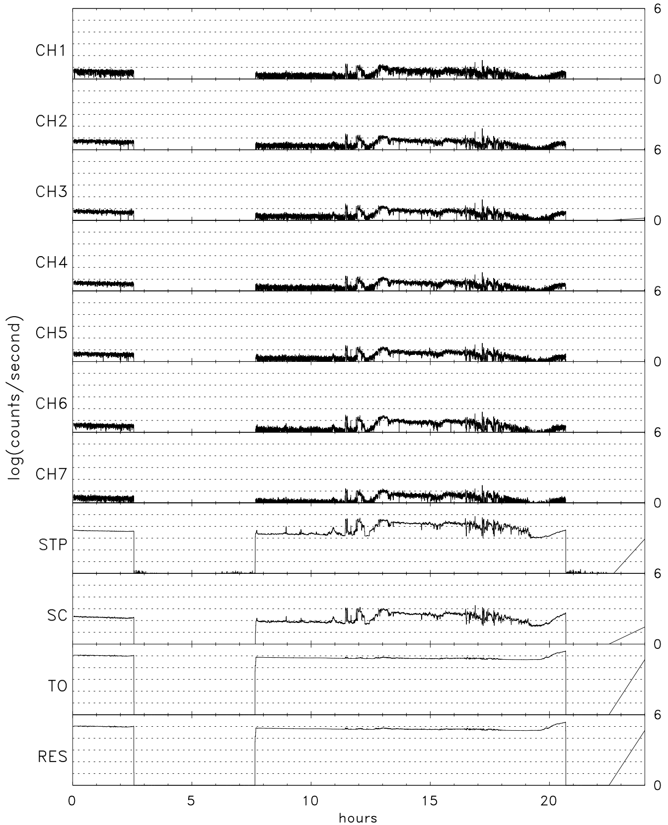
TIDE energy/spin averaged H+ for 12/08/06 (342)
