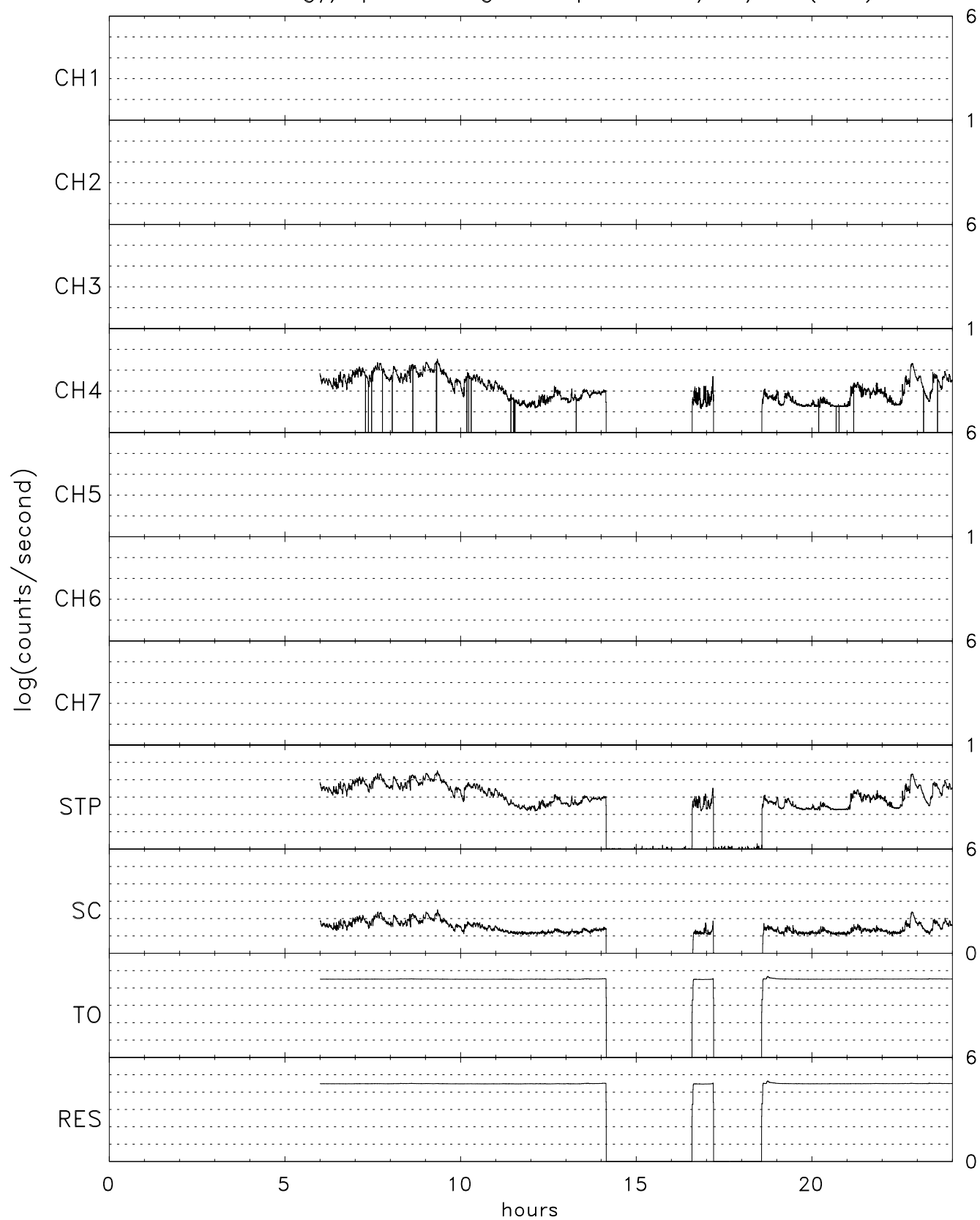
TIDE energy/spin averaged Stops for 12/06/06 (340)
