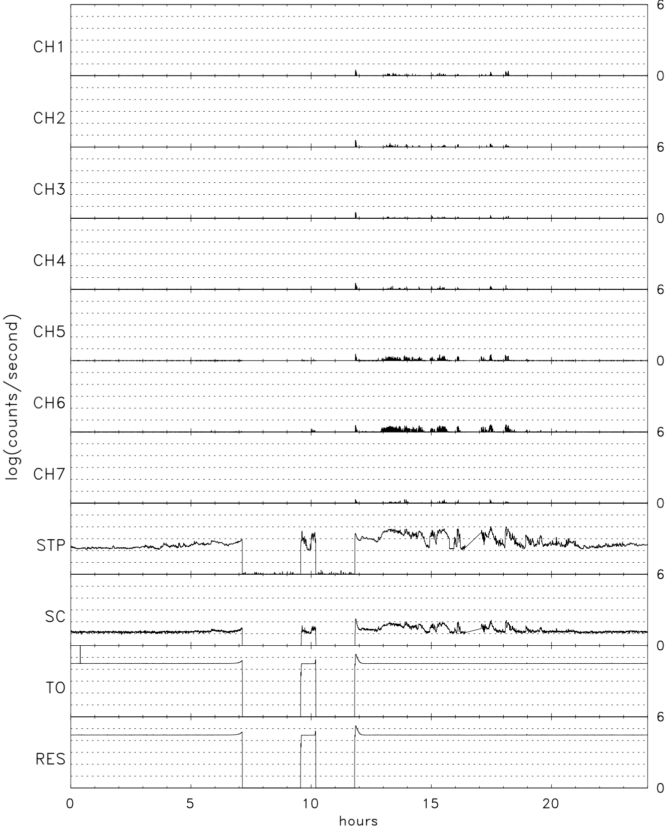
TIDE energy/spin averaged 0+ for 12/04/06 (338)
