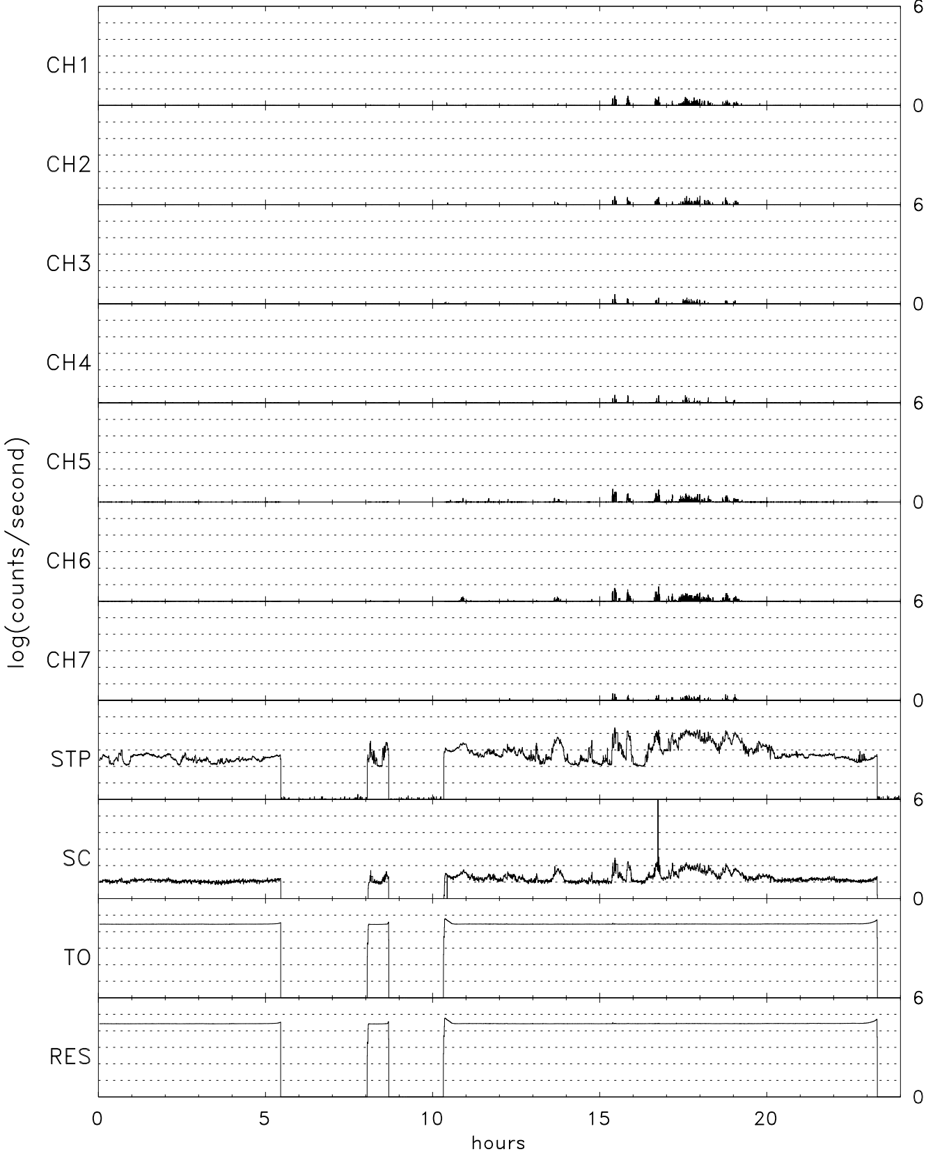
TIDE energy/spin averaged H+ for 12/01/06 (335)
