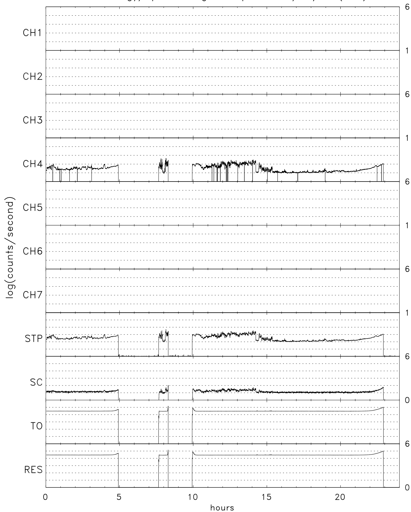
TIDE energy/spin averaged Stops for 11/18/06 (322)
