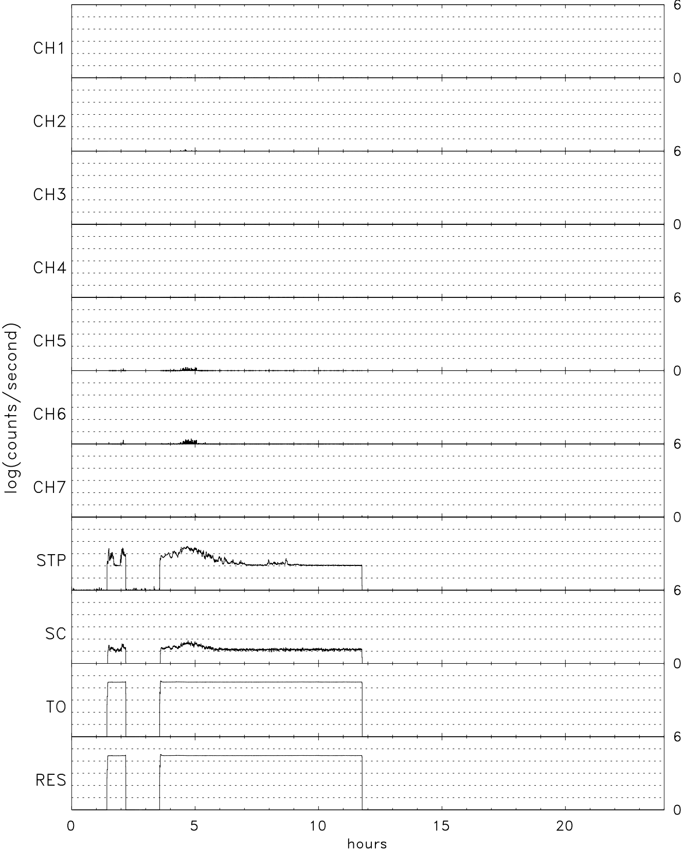
TIDE energy/spin averaged 0+ for 11/06/06 (310)
