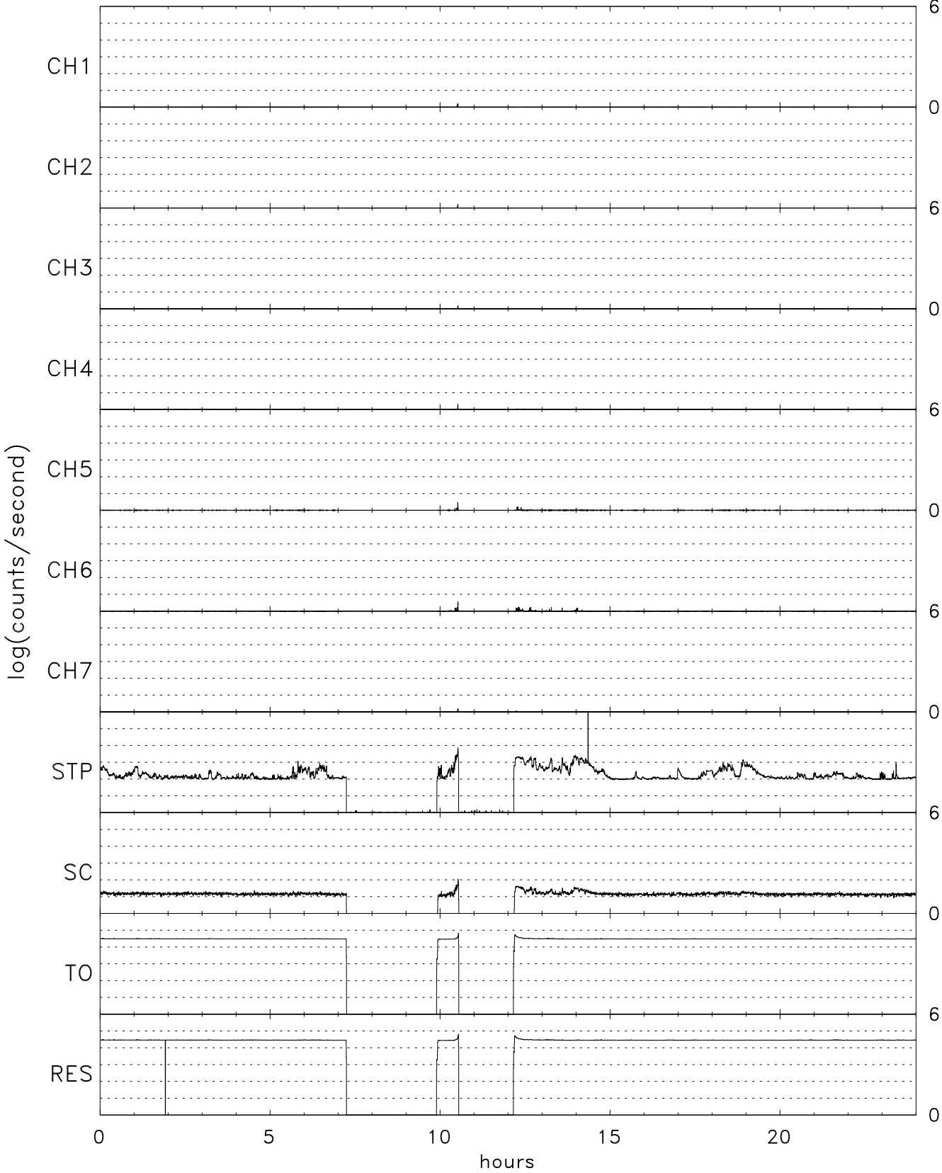
TIDE energy/spin averaged 0+ for 10/29/06 (302)
