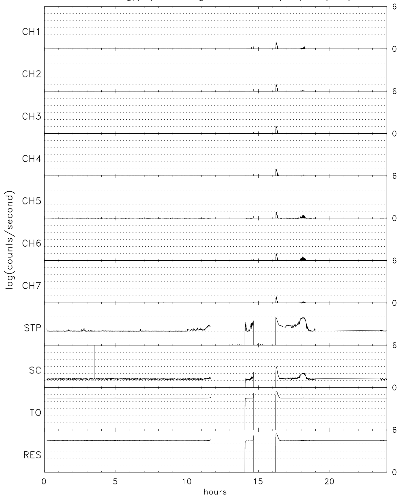
TIDE energy/spin averaged He+ for 10/25/06 (298)
