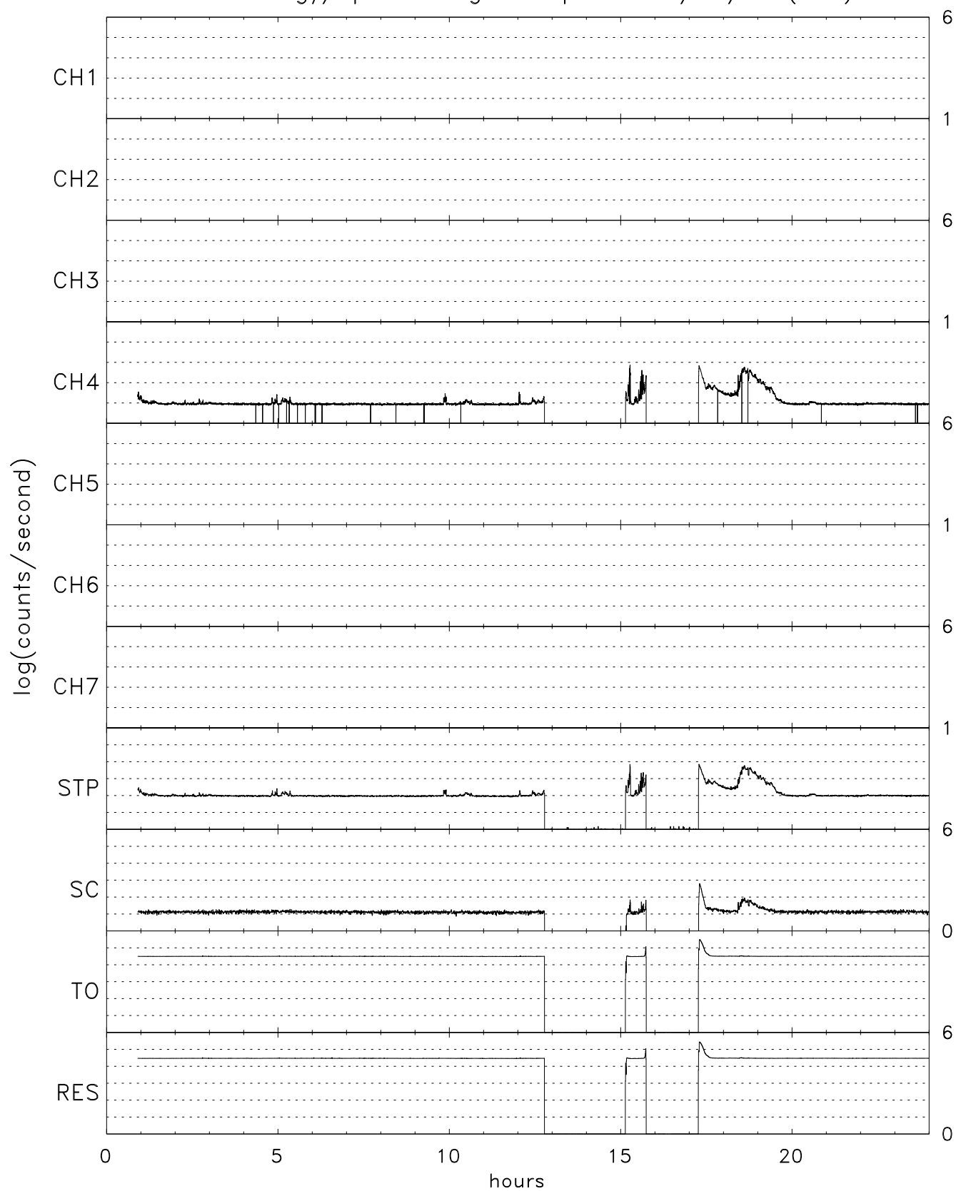
TIDE energy/spin averaged Stops for 10/15/06 (288)
