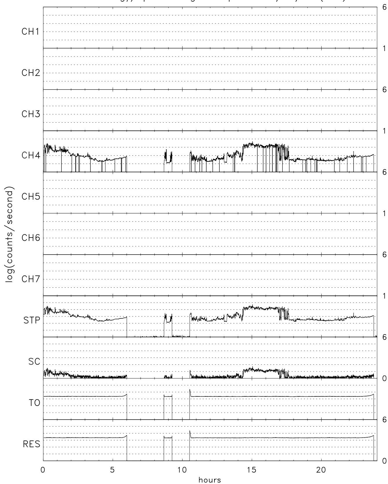
TIDE energy/spin averaged Stops for 01/08/06 (008)
