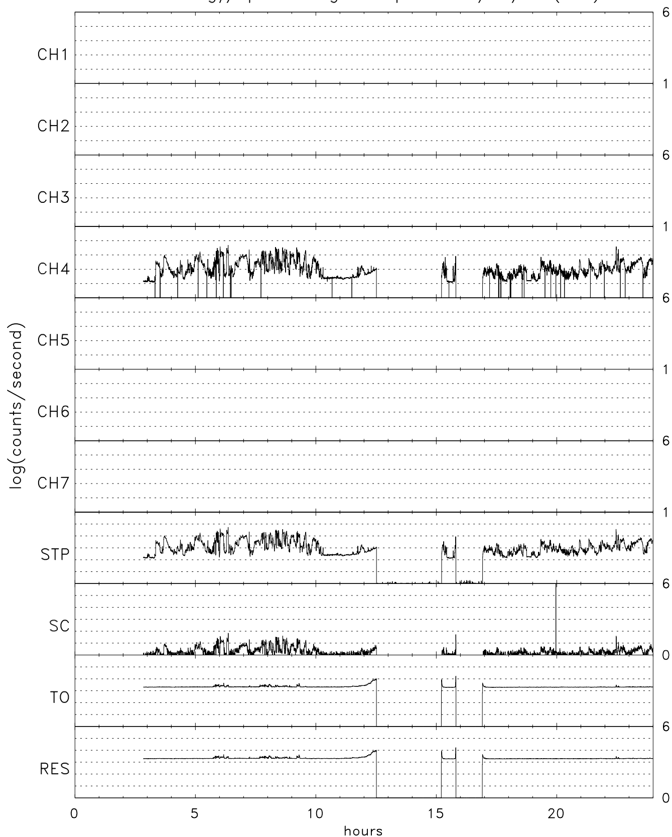
TIDE energy/spin averaged Stops for 12/28/05 (362)
