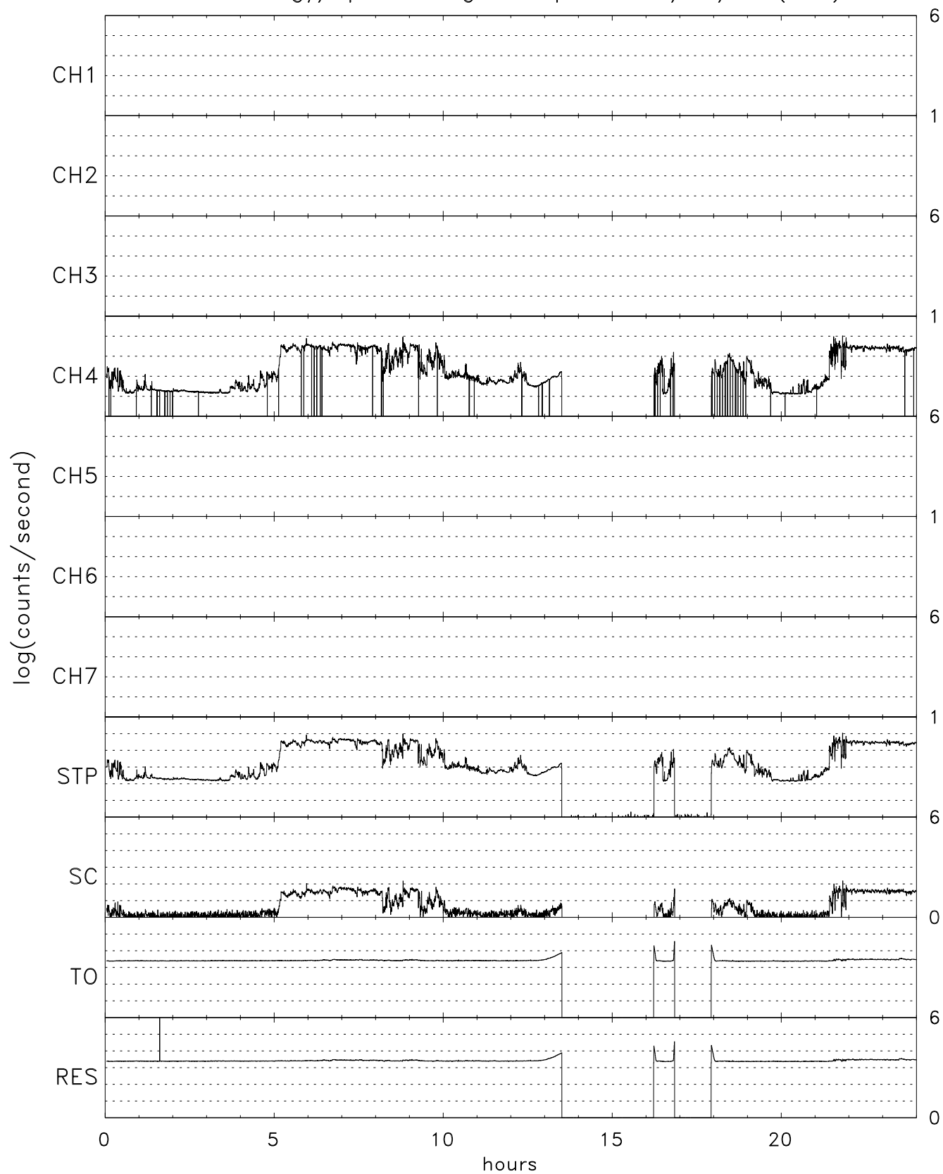
TIDE energy/spin averaged Stops for 12/18/05 (352)
