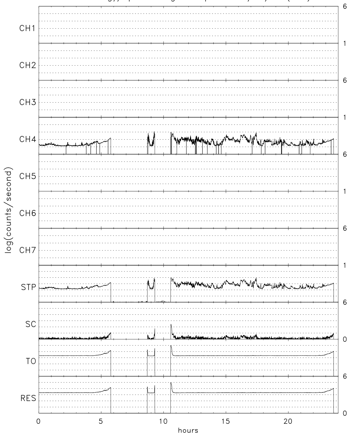
TIDE energy/spin averaged Stops for 12/03/05 (337)
