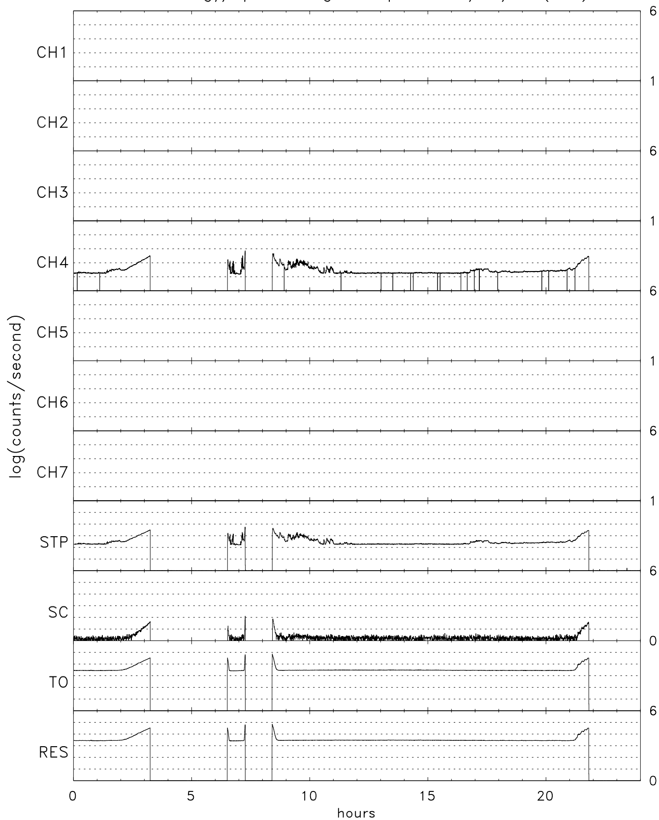
TIDE energy/spin averaged Stops for 10/12/05 (285)
