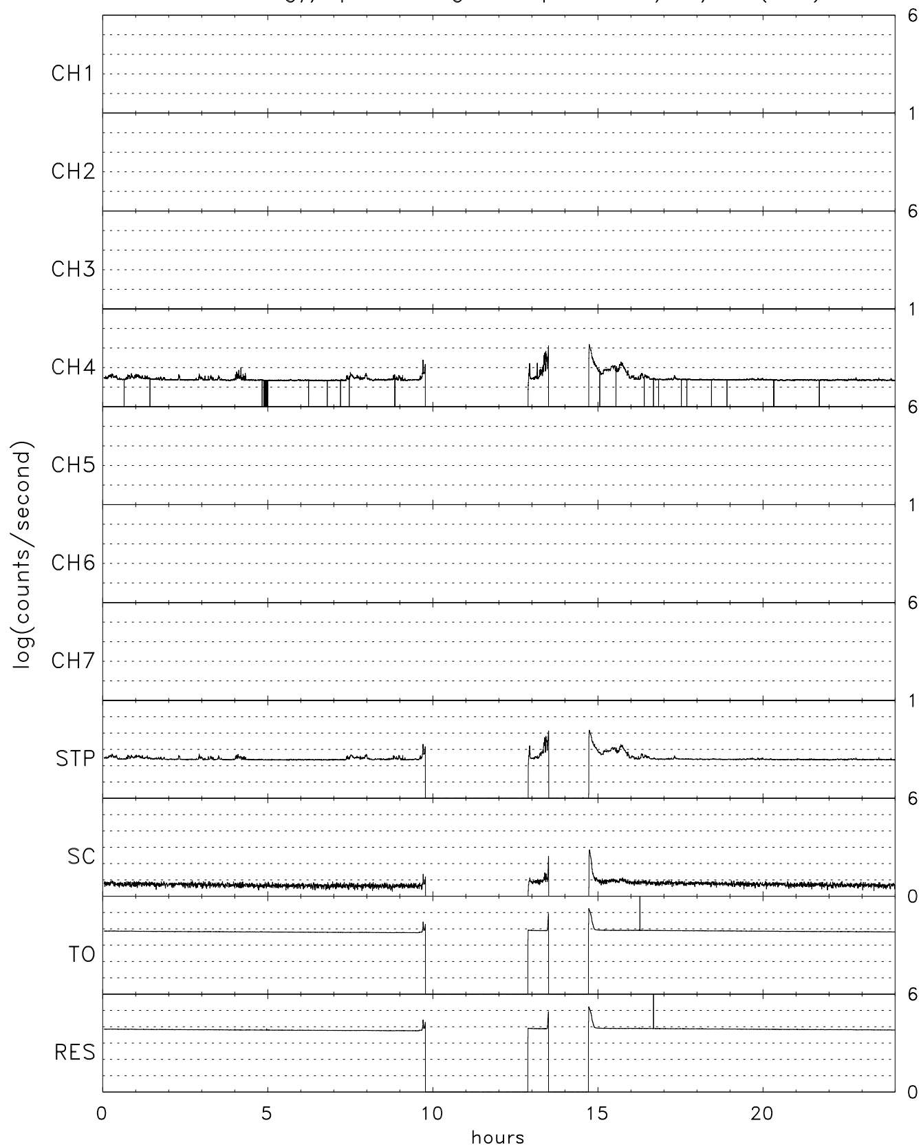
TIDE energy/spin averaged Stops for 09/18/05 (261)
