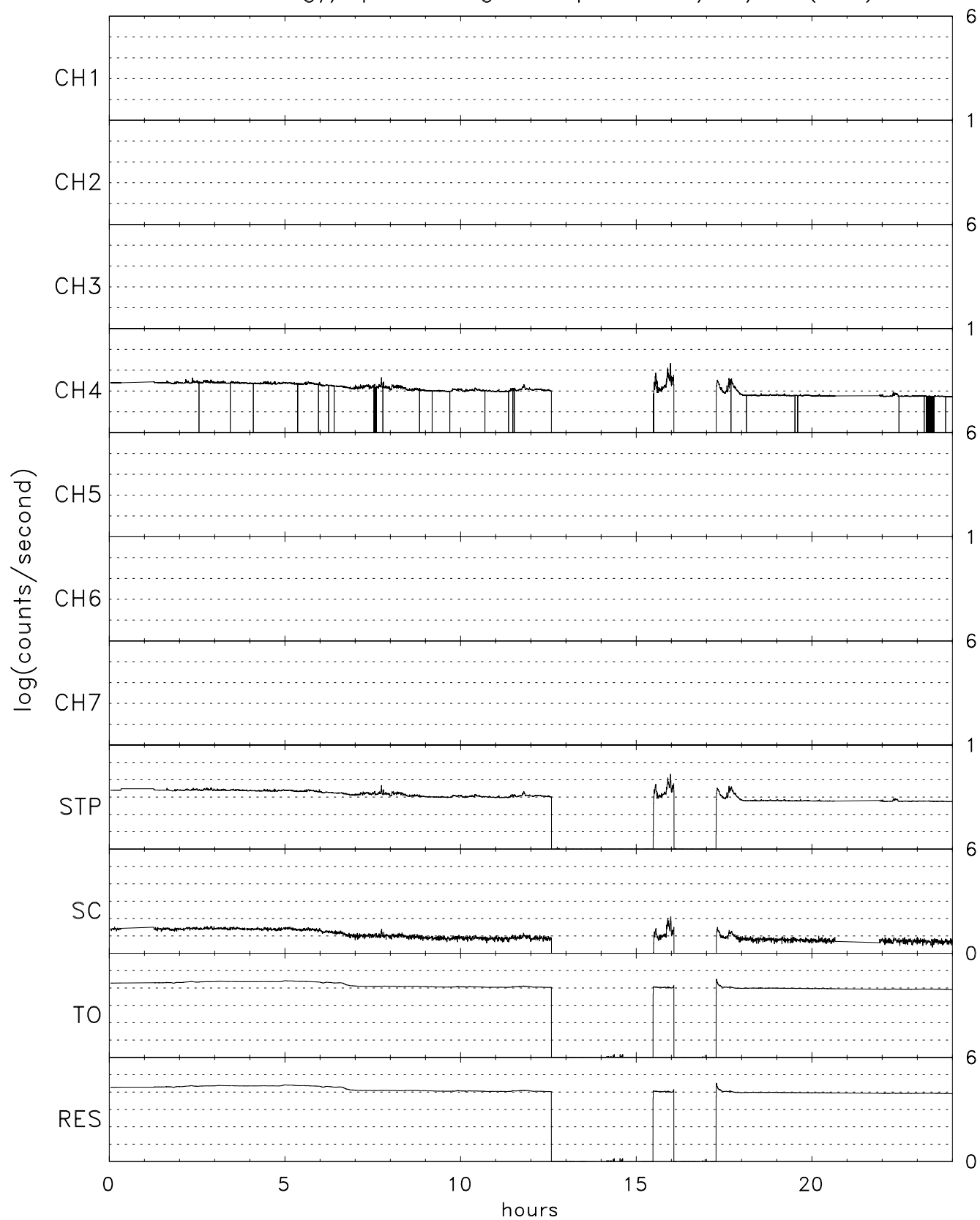
TIDE energy/spin averaged Stops for 09/11/05 (254)
