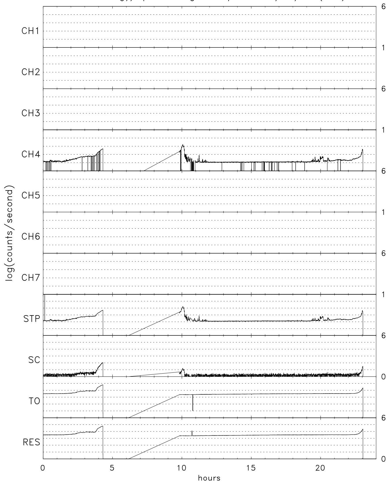
TIDE energy/spin averaged Stops for 08/27/05 (239)
