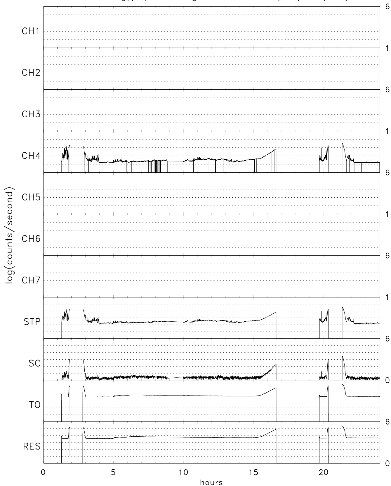
TIDE energy/spin averaged Stops for 06/27/05 (178)
