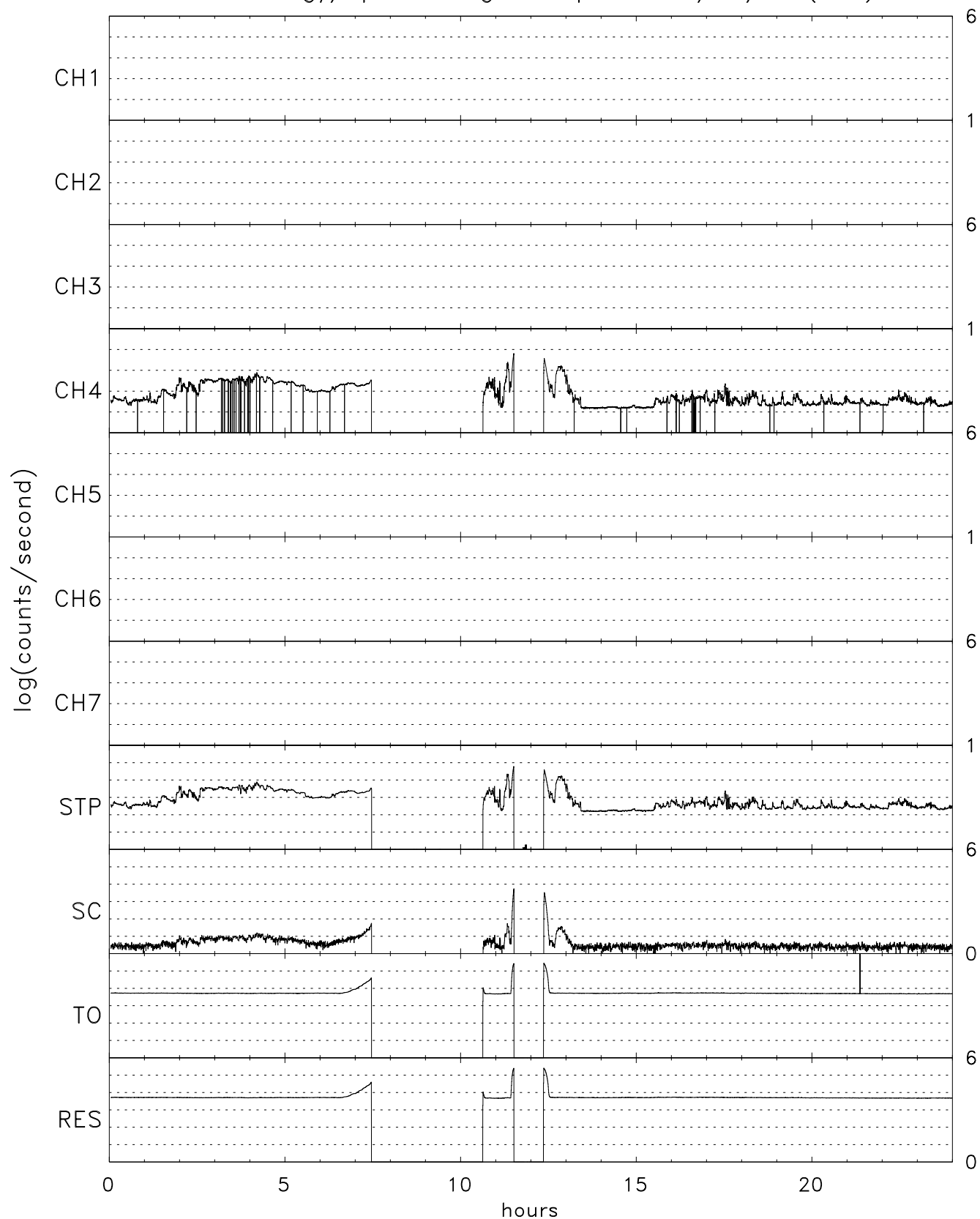
TIDE energy/spin averaged Stops for 06/22/05 (173)
