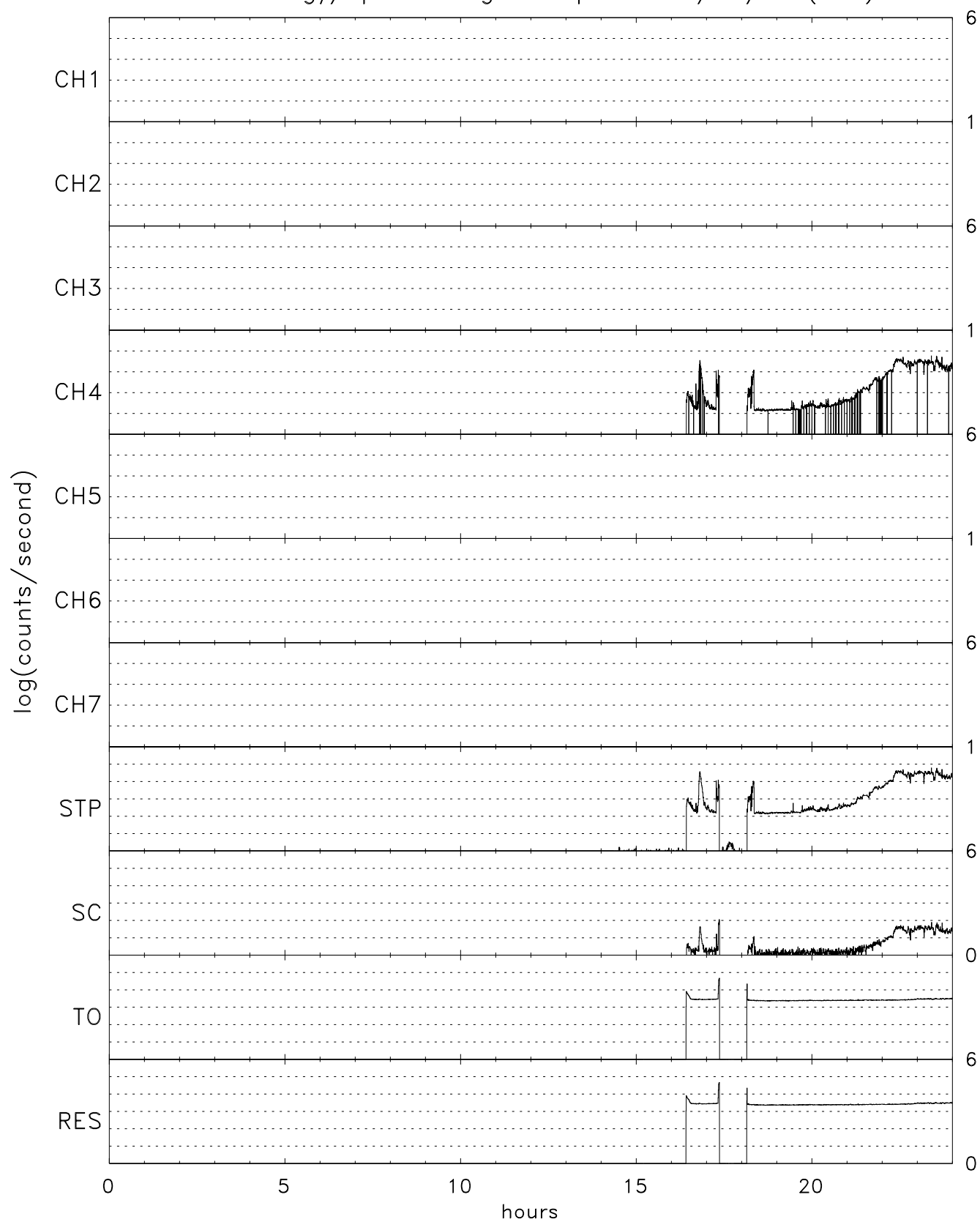
TIDE energy/spin averaged Stops for 03/05/05 (064)
