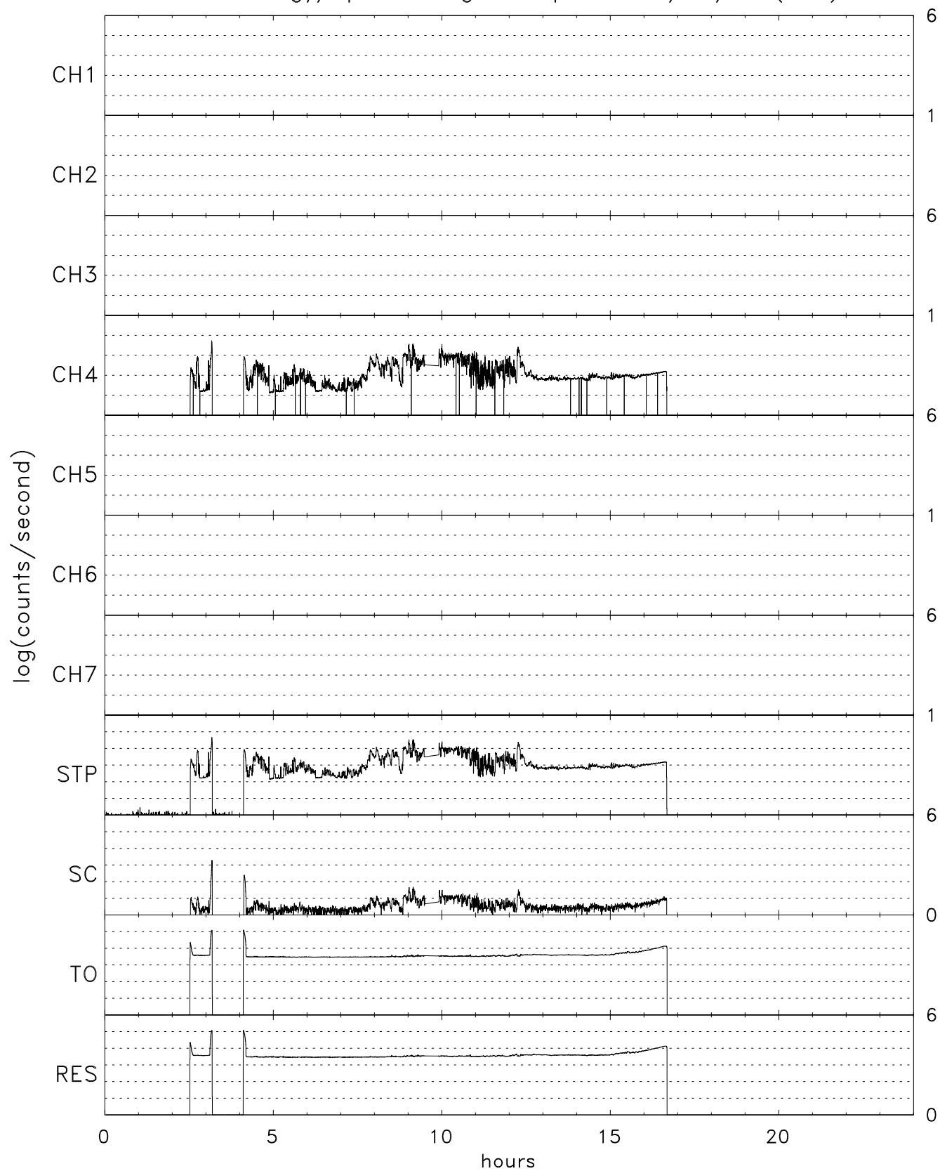
TIDE energy/spin averaged Stops for 03/01/05 (060)
