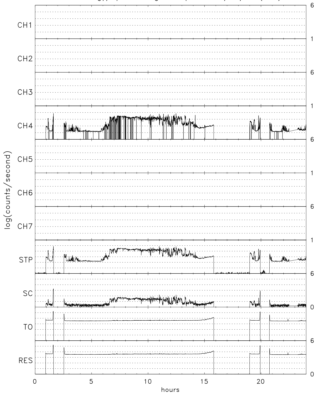
TIDE energy/spin averaged Stops for 02/26/05 (057)
