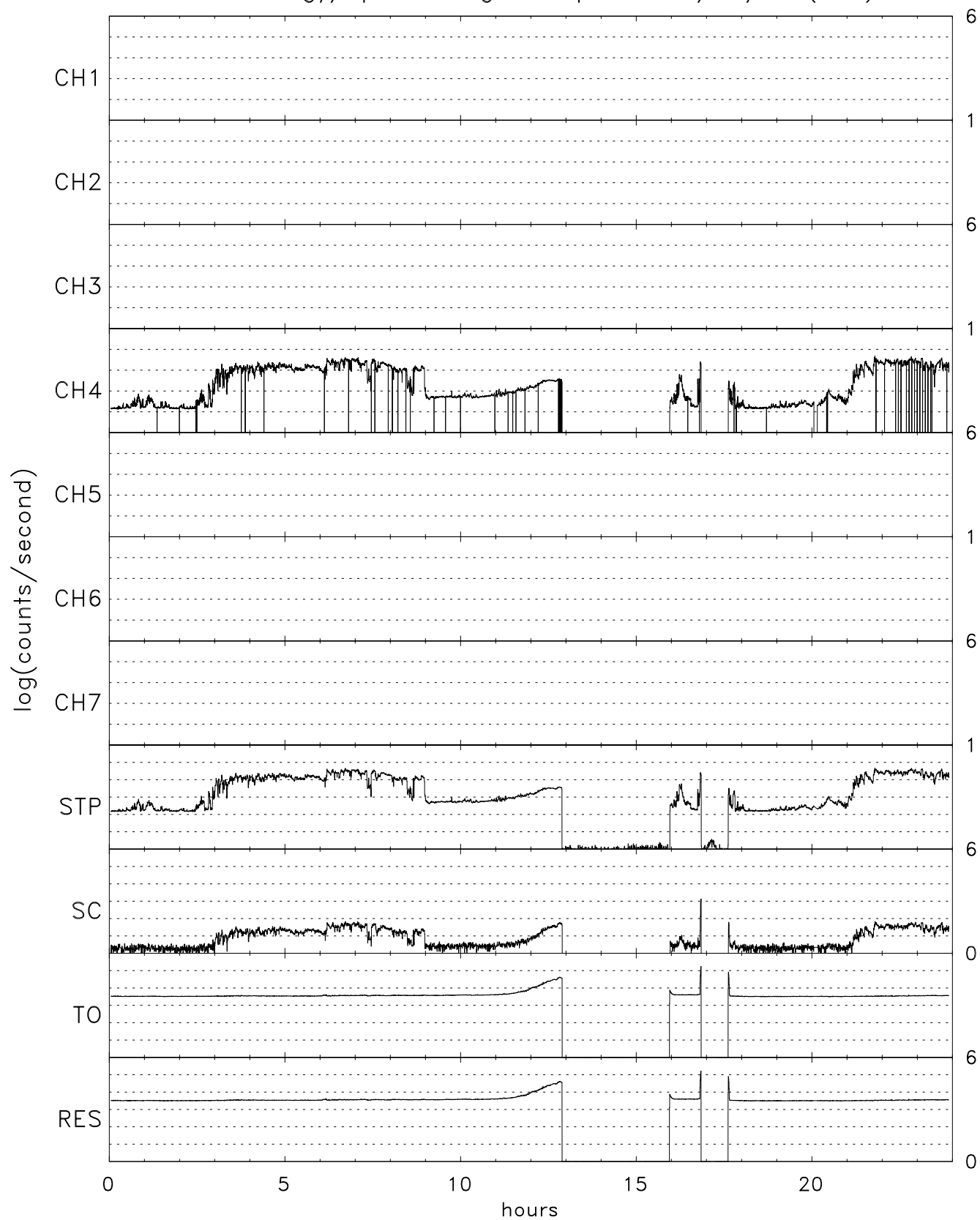
TIDE energy/spin averaged Stops for 02/20/05 (051)
