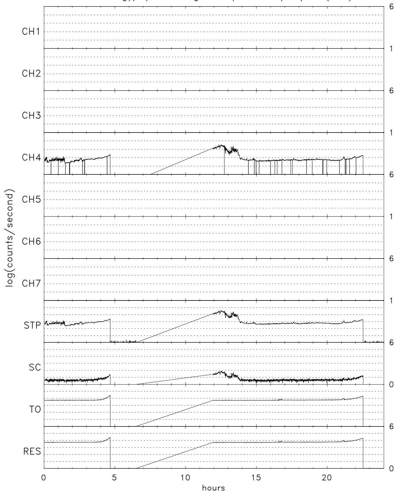
TIDE energy/spin averaged Stops for 02/15/05 (046)
