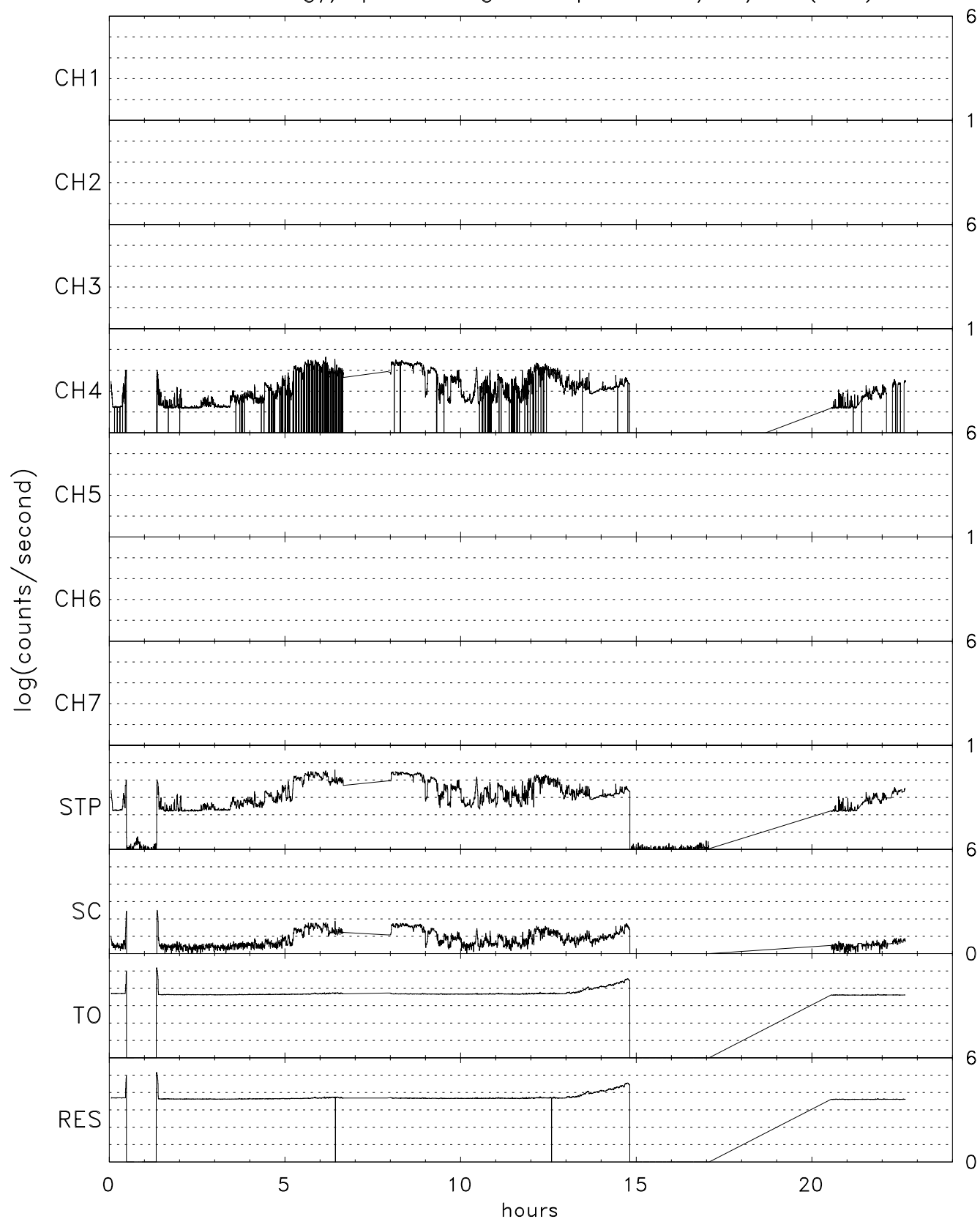
TIDE energy/spin averaged Stops for 01/31/05 (031)
