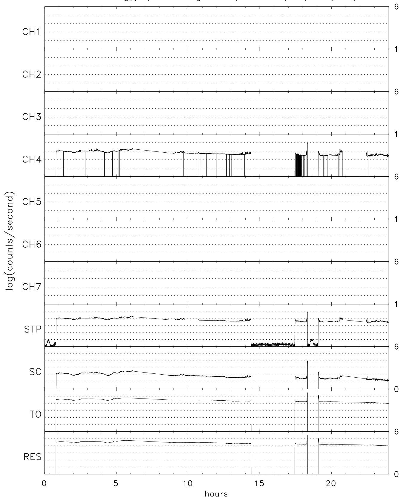
TIDE energy/spin averaged Stops for 01/18/05 (018)
