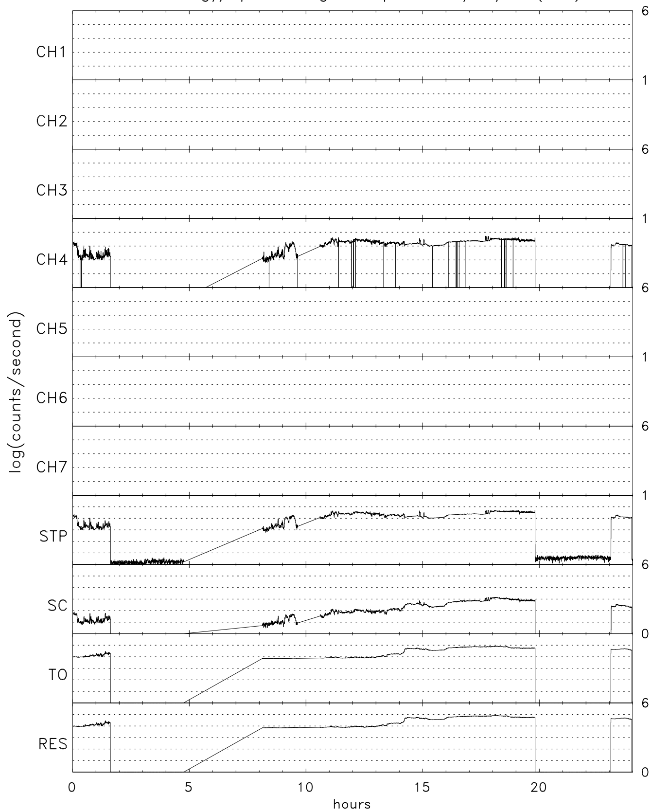
TIDE energy/spin averaged Stops for 01/17/05 (017)
