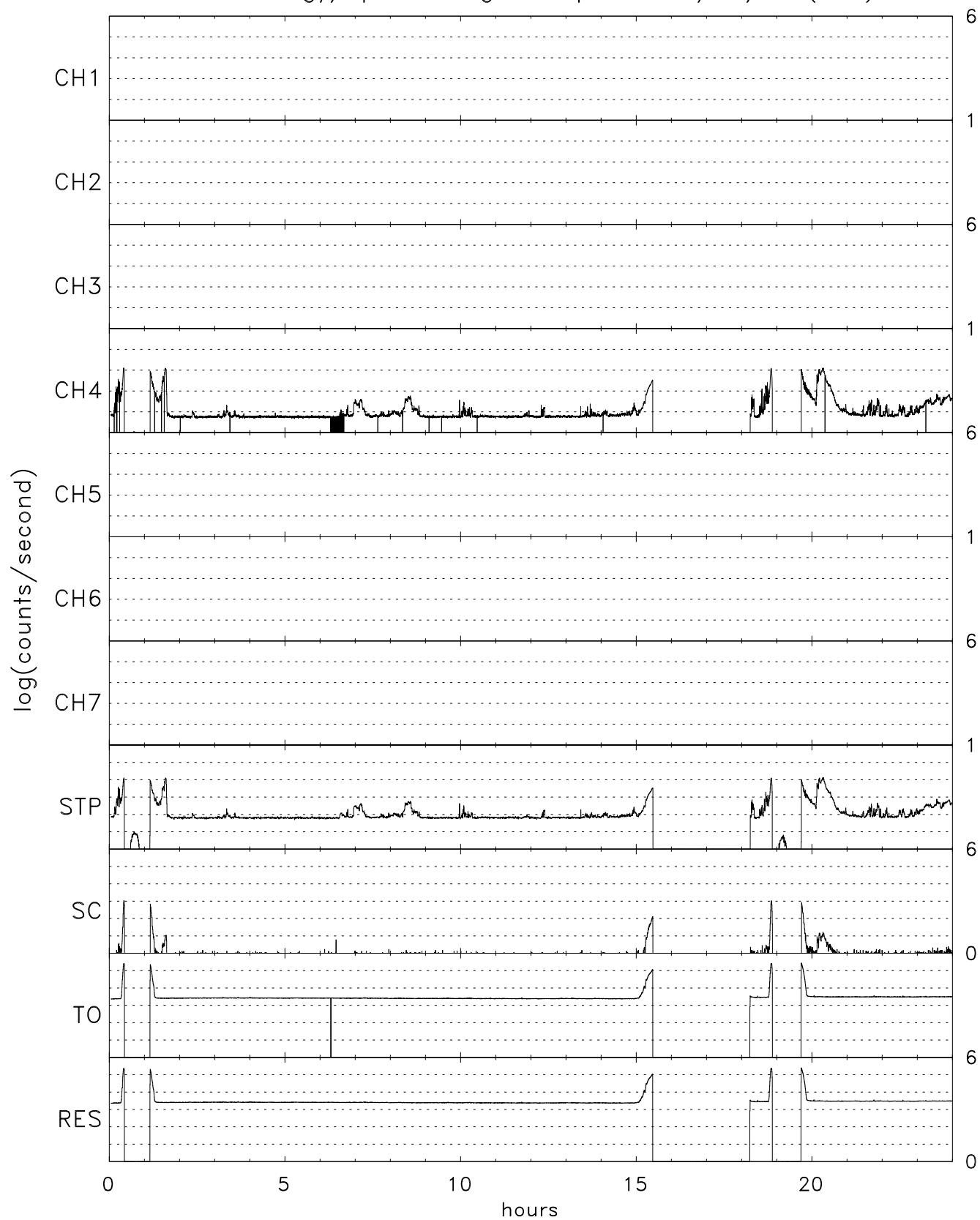
TIDE energy/spin averaged Stops for 10/15/04 (289)
