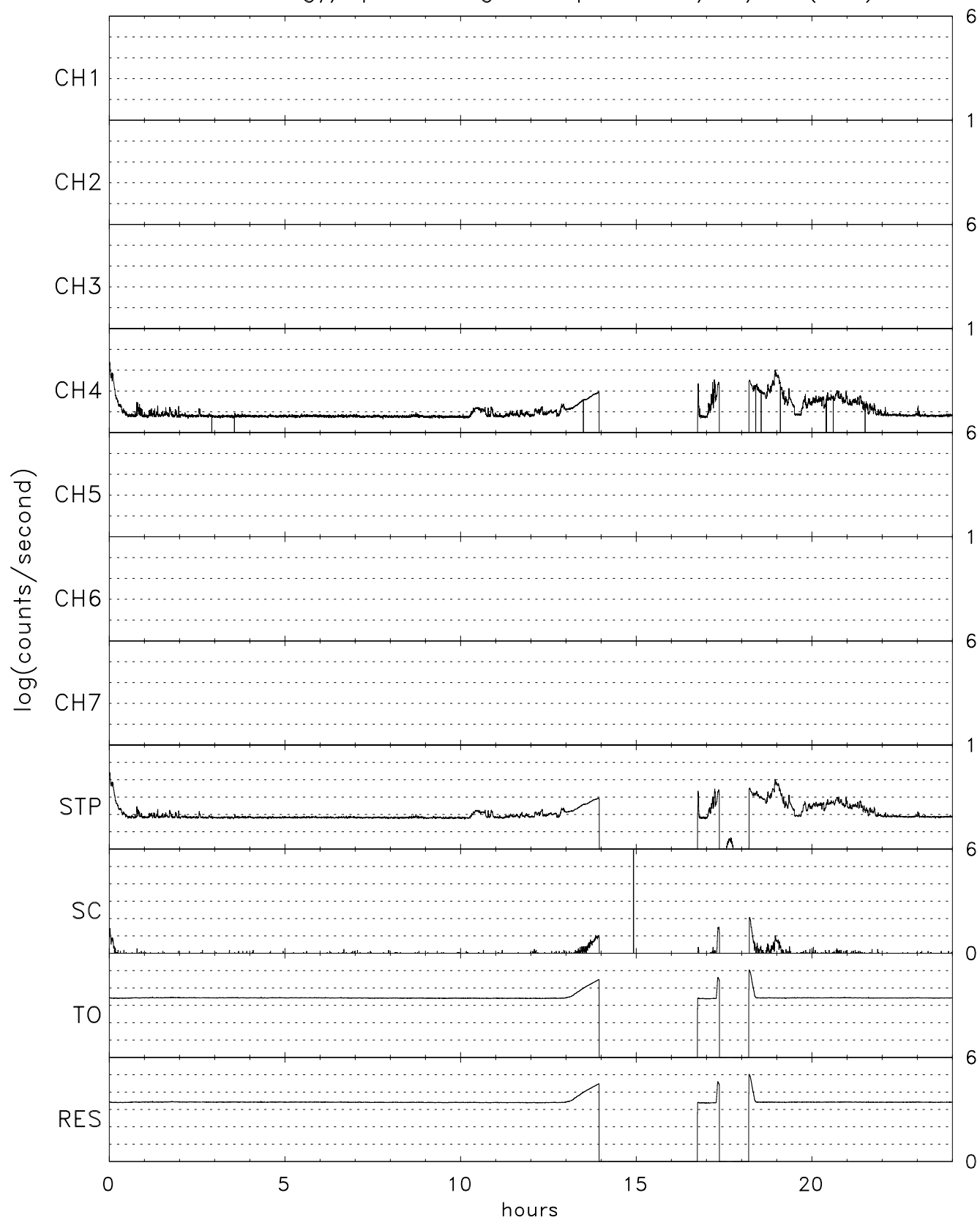
TIDE energy/spin averaged Stops for 10/12/04 (286)
