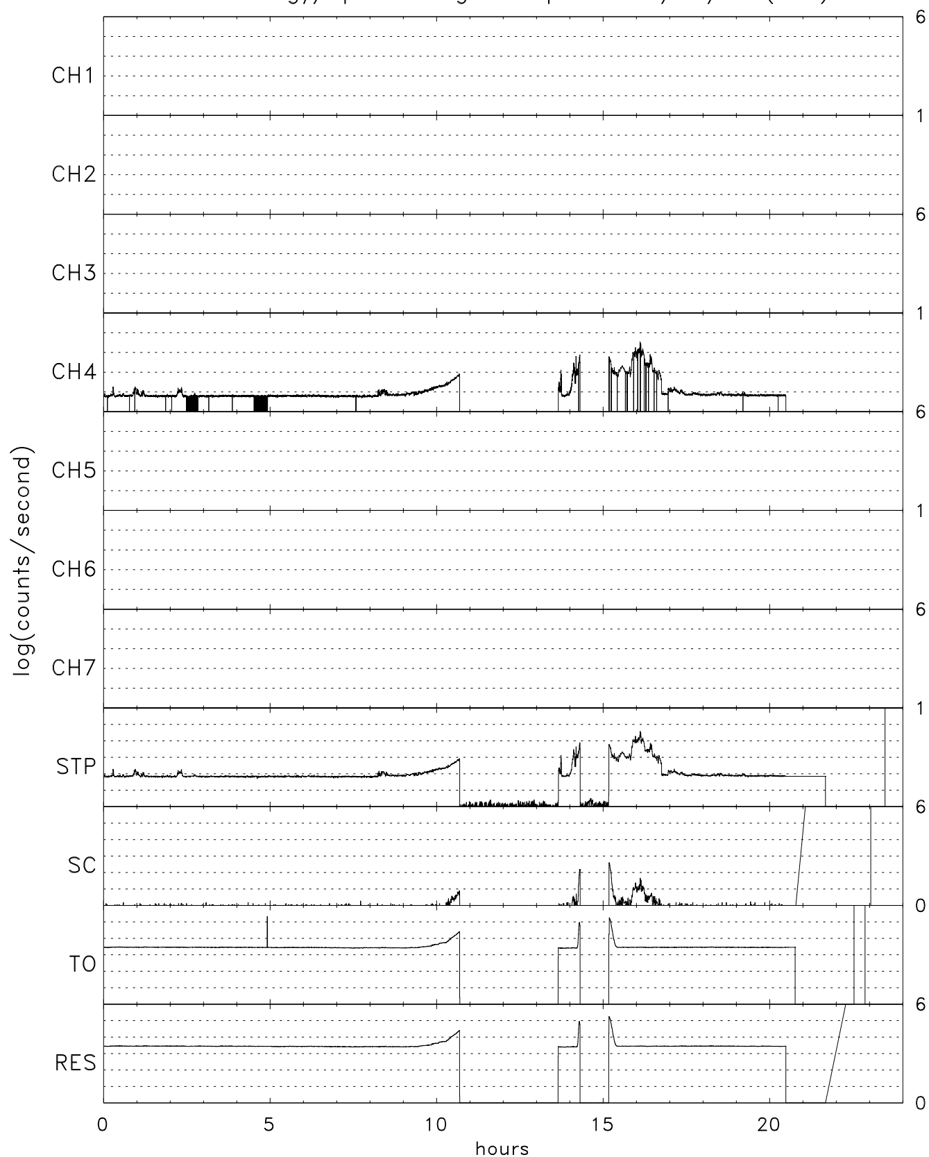
TIDE energy/spin averaged Stops for 10/06/04 (280)
