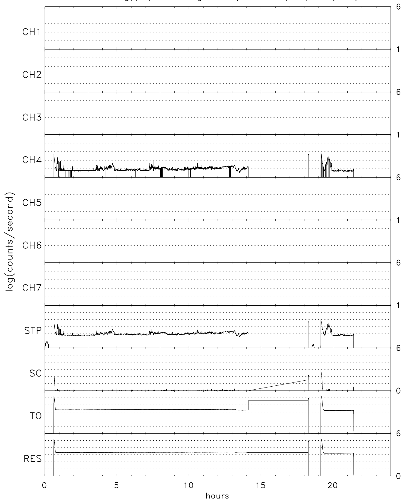
TIDE energy/spin averaged Stops for 08/27/04 (240)
