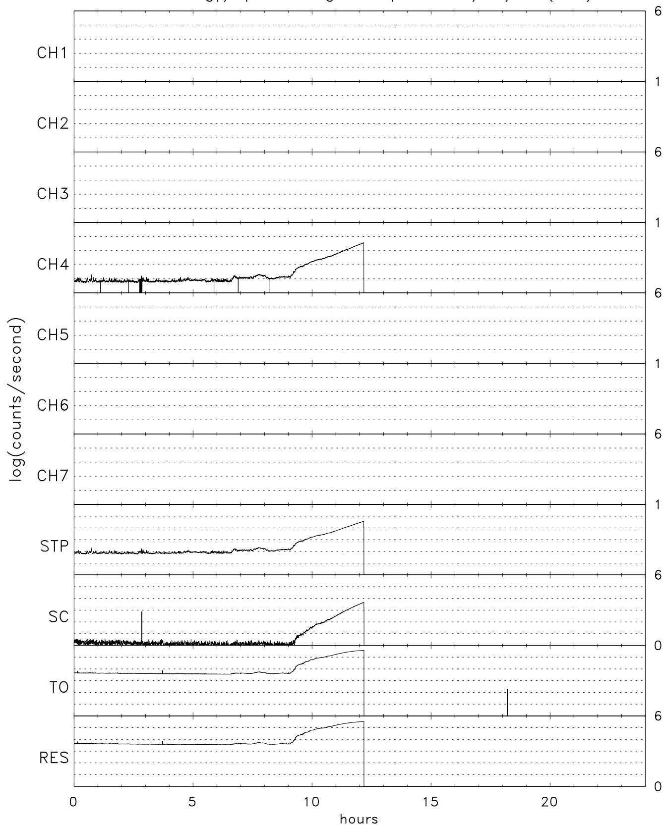
TIDE energy/spin averaged Stops for 07/29/04 (211)
