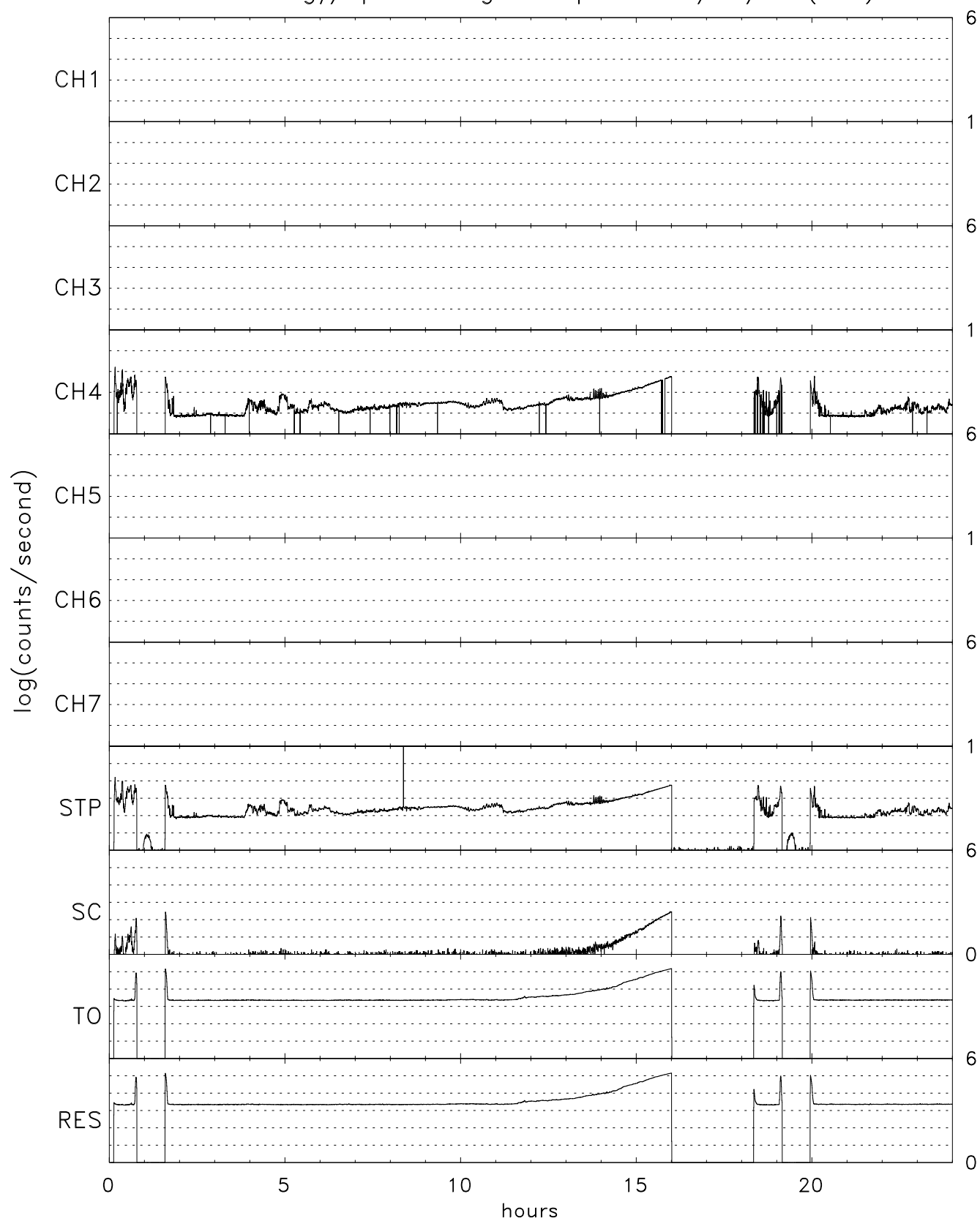
TIDE energy/spin averaged Stops for 06/06/04 (158)
