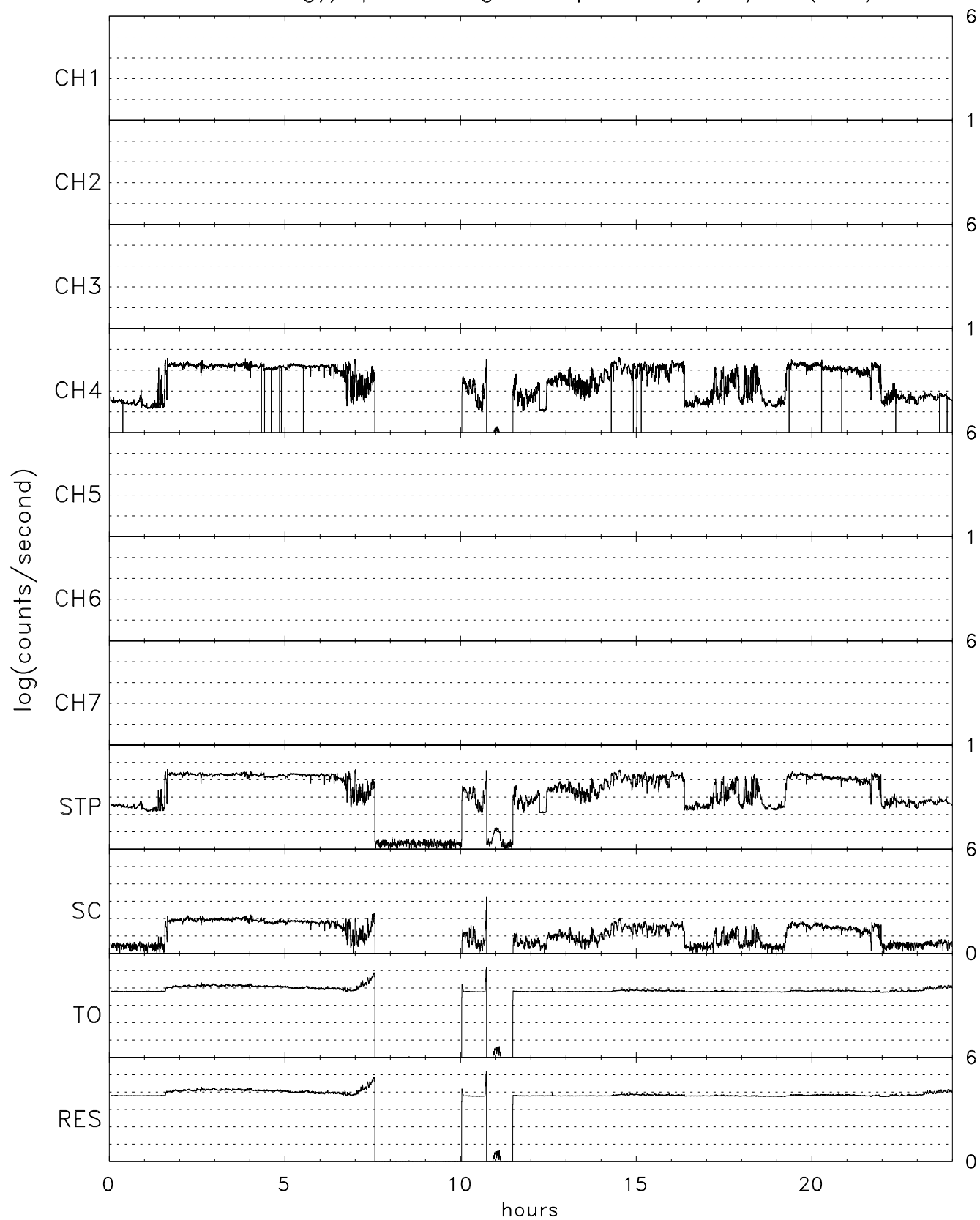
TIDE energy/spin averaged Stops for 01/22/04 (022)
