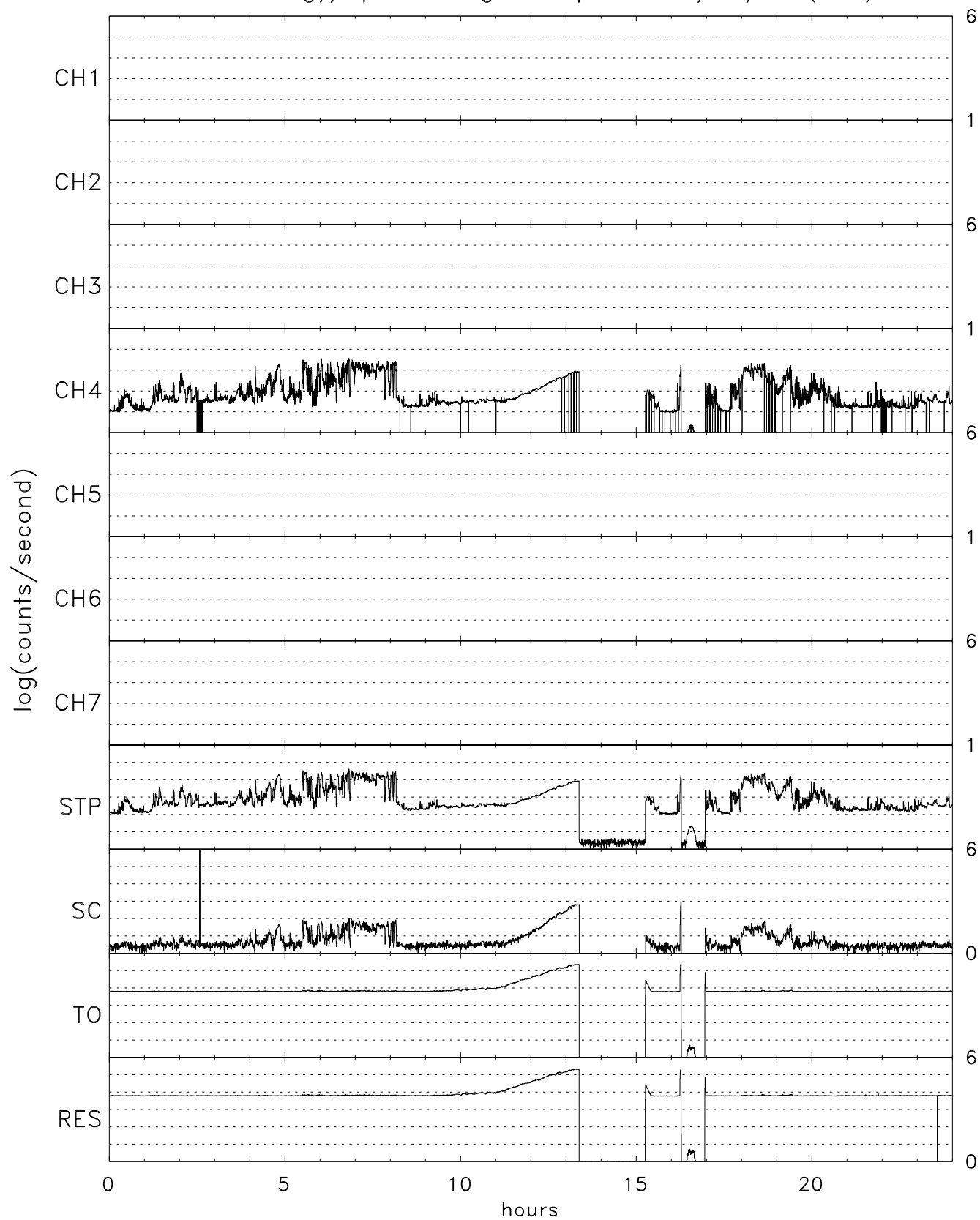
TIDE energy/spin averaged Stops for 01/21/04 (021)
