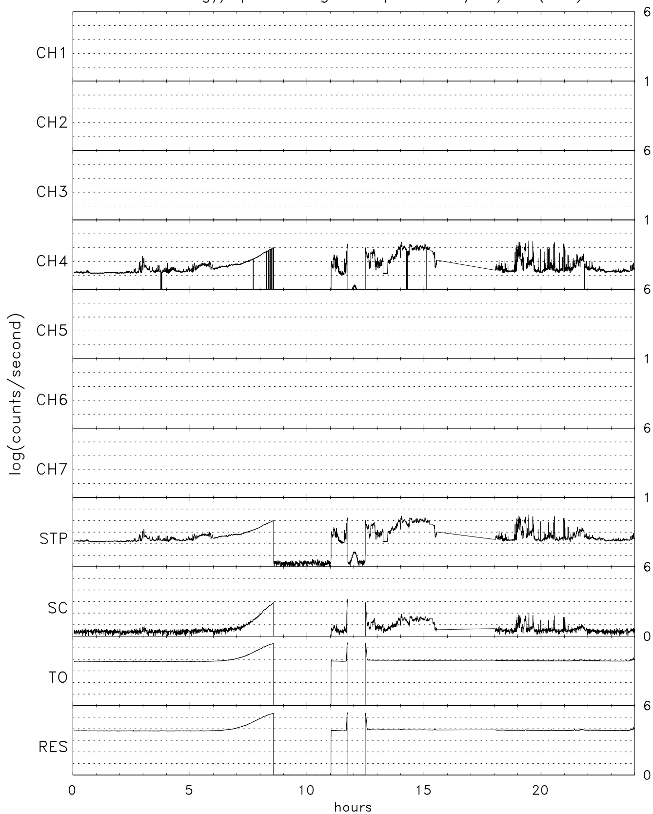
TIDE energy/spin averaged Stops for 01/12/04 (012)
