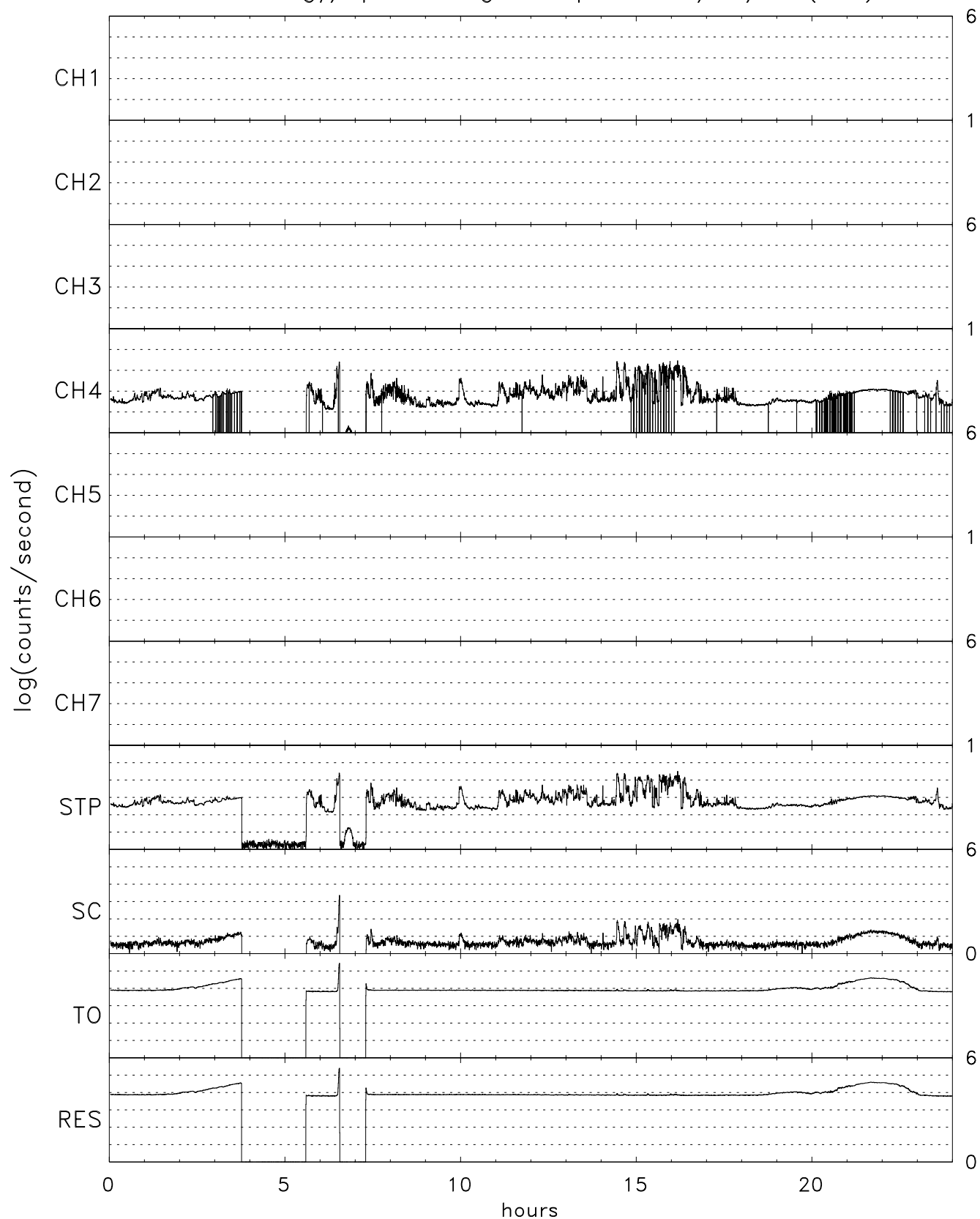
TIDE energy/spin averaged Stops for 12/21/03 (355)
