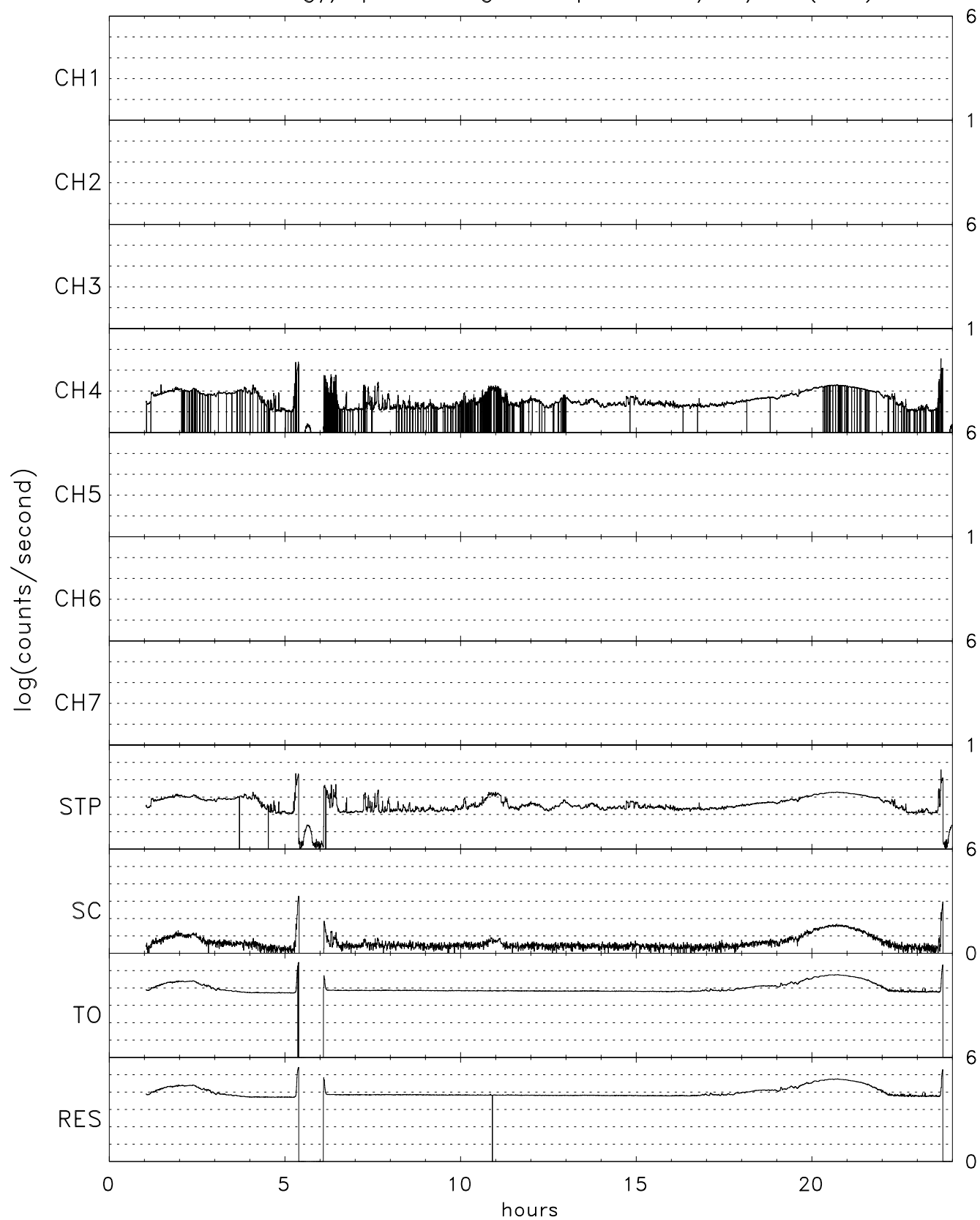
TIDE energy/spin averaged Stops for 11/25/03 (329)
