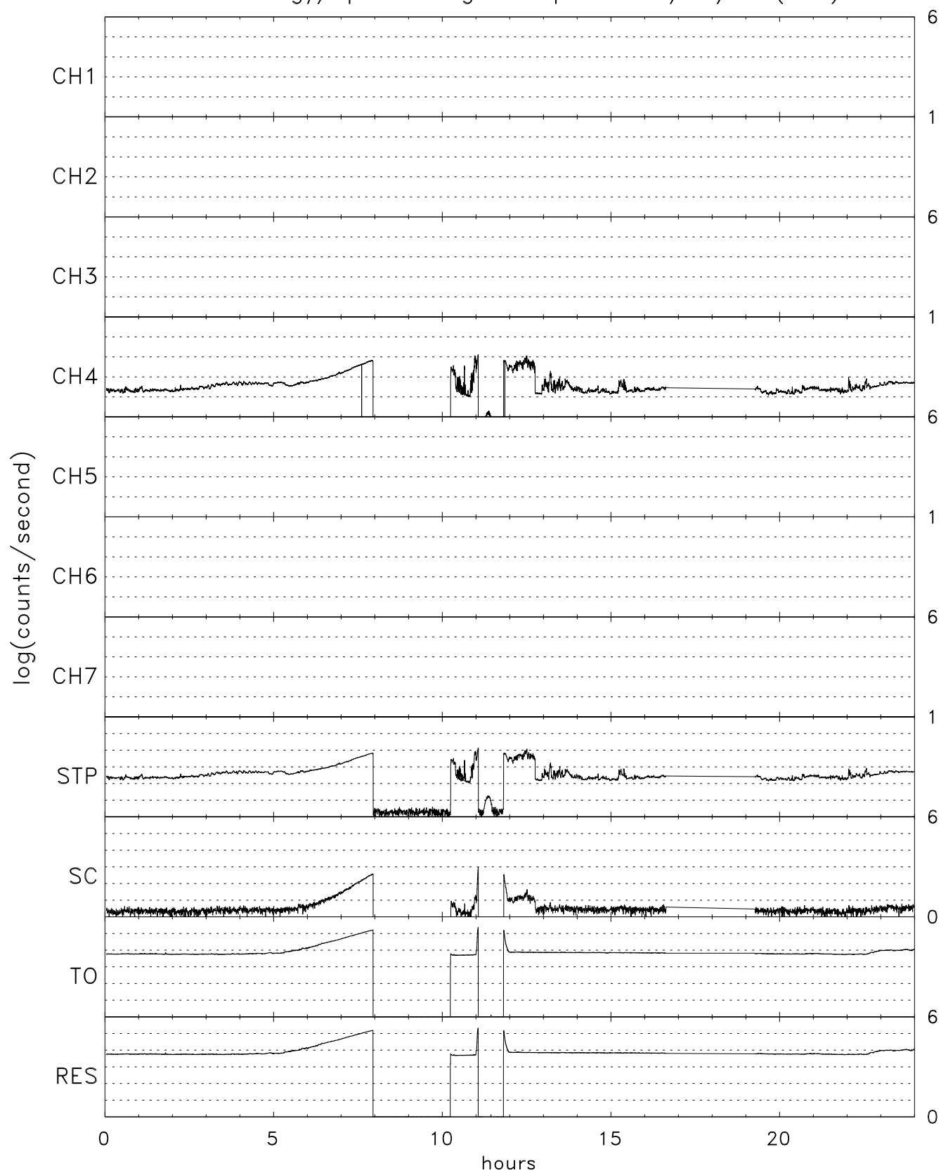
TIDE energy/spin averaged Stops for 11/24/03 (328)
